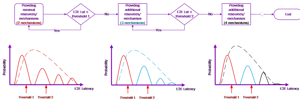
FIGURE 2.11: Multi step decision making process.
