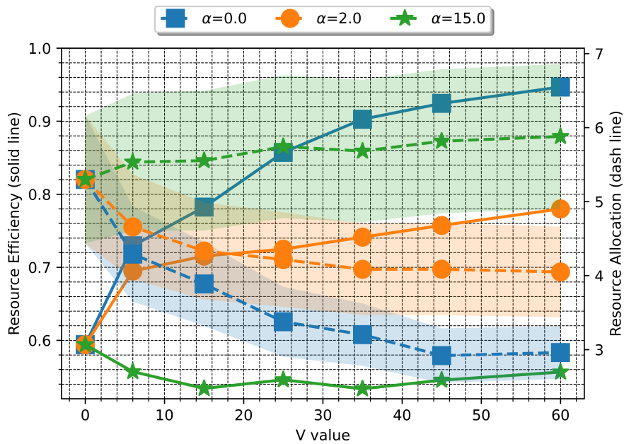
FIGURE 3.16: Resource allocation and efficiency
