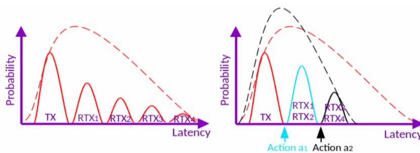
FIGURE 3.9: Early decision making scheme
