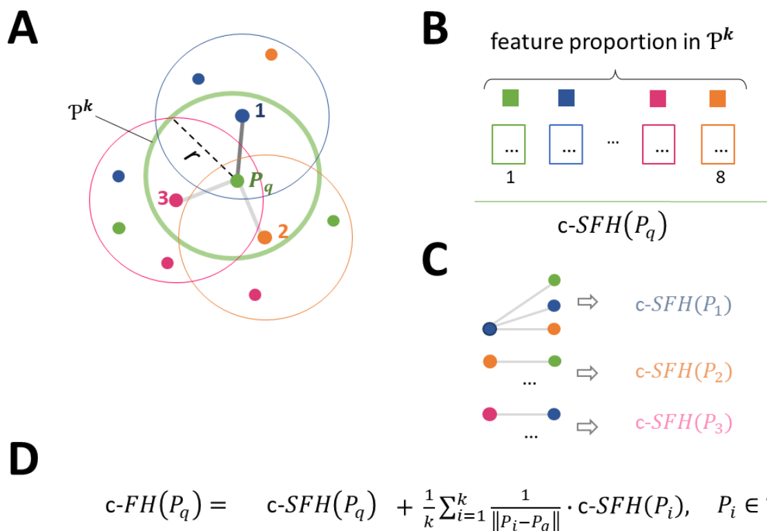
Figure S2. Colored Feature Histogram (c-FH descriptor) 2 used to align sc-PDB subpockets to the target cavity. A ) Considering a point P_q (green) whose c-FH is to be computed, its neighbor points \mathcal{P}^k = \{1, 2, 3\} within a radius r are determined (green circle). For each neighbor in \mathcal{P}^k , their respective neighbors are also determined within the radius r . B ) The percentage of each of eight pharmacophoric features (hydrophobic, aromatic, H-bond donor, H-bond acceptor, H-bond acceptor and donor, positive ionizable, negative ionizable, null) is then stored into a 8-bin histogram that forms the simplified colored feature histogram (c-SFH) of the point P_q . C ) The c-SFH is iteratively computed for each point in \mathcal{P}^k ; D ) The c-FH of the point P_q is the sum of its c-SFH and the distance-weighted average of its neighbors' c-FSHs.
