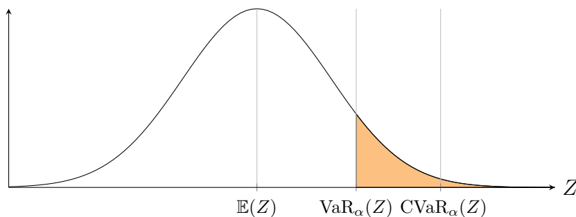
Figure 7.1: Value-at-risk and Conditional Value-at-risk at confidence level \alpha = 0.95 for a normally distributed random variable
