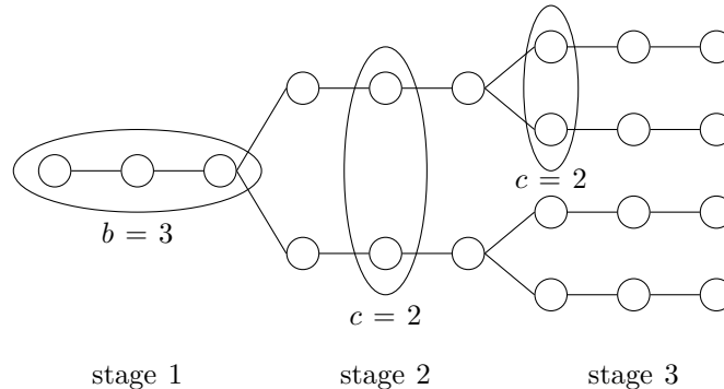
Figure 3.2: Scenario tree structure
