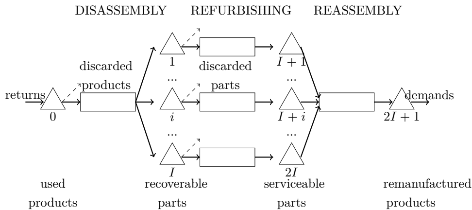
Figure 3.1: Illustration of studied remanufacturing system
