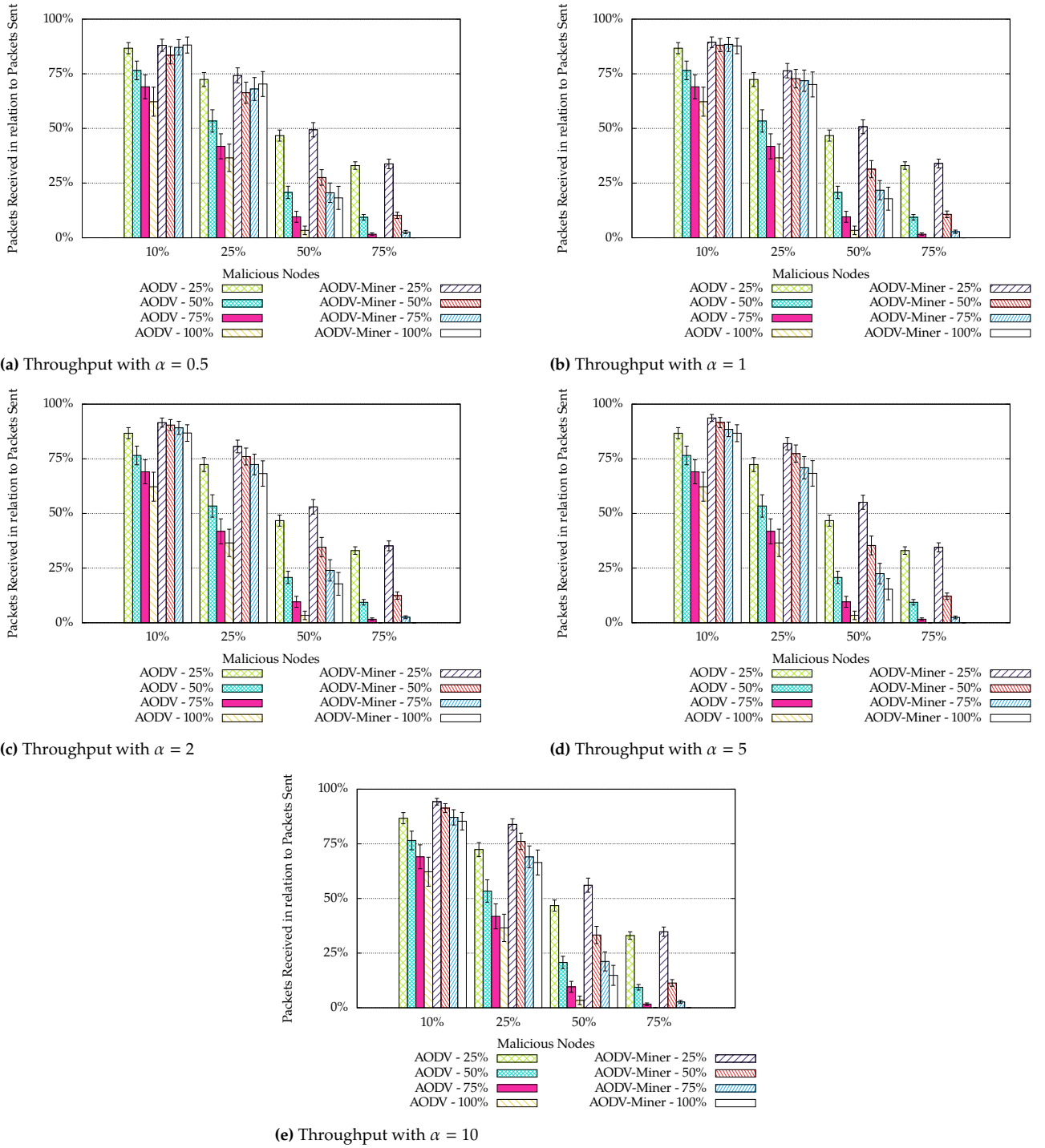
Figure 4.26: Throughput comparison between AODV-Miner and AODV in a network of 30 nodes, subjected to varying probability Grey-hole attacks
