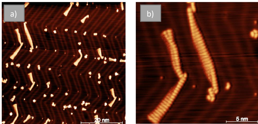
Figure 4. 8 : a) STM topographic image of BDPA on Au(111) at 32 K (1 V/10 pA). The observed broadening results from the transverse mechanical vibrations of BDPA molecules. b) Zoom on a BDPA chain at 32 K where different modes of vibrations are observed (1 V/10 pA).
