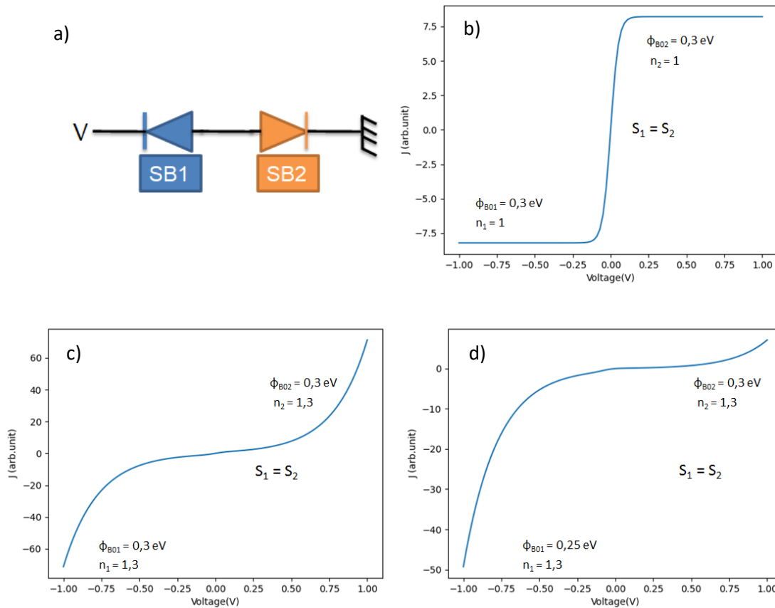
Figure 3. 9 : a) Equivalent circuit modeled by Eq. (3. 5). b) Simulated I-V characteristics for contact using \phi_{B01} = \phi_{B02} = 0.3 V, the same junction area S_1 = S_2 , and a perfect ideality factor ( n=1 ). c) Simulated characteristics, introducing an ideality factor n=1.3 . c) Simulated I-V characteristic using asymmetric barrier heights \phi_{B01}=0.25 V, \phi_{B02} = 0.3 V, S_1 = S_2 , and an ideality factor n=1.3 .
