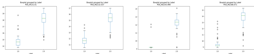
Figure 4: Boxplots concerning relative abundances of features POS_131.0342, POS_132.0375 POS_243.9903 and POS_166.0712 of the BRAIN dataset, most likely corresponding to different adducts of 2-Hydroxyglutarate. Fold changes : 32.9, 35.6, 14.6 and 33.7 respectively. Label 1 : samples of tumors with wild type IDH, Label 2 : samples of tumors with mutated IDH.
