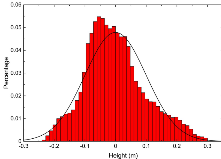
Figure 2.4: Histogram of the height distribution of our generated isotropic self-affine surface at the 512 m scale, with Hurst exponent H = 0.8 and roughness amplitude h_{rms} = 0.1 m, consistent with the field observations of Candela et al. (2012) (see blue circles in Fig. 1). The largest height fluctuations are on the order of 3h_{rms} \approx \pm 0.3 m for a lateral extension of 512 m
