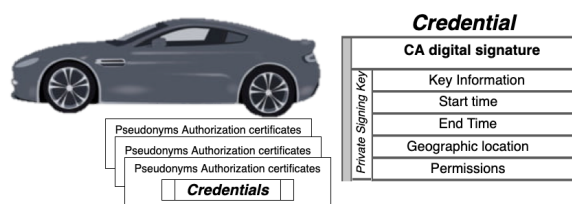
Fig. 3.1 Credential composition
