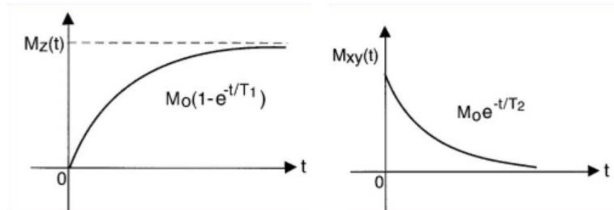
Fig. 1.3 Schema for T1 relaxation (left) and T2 relaxation (right).
