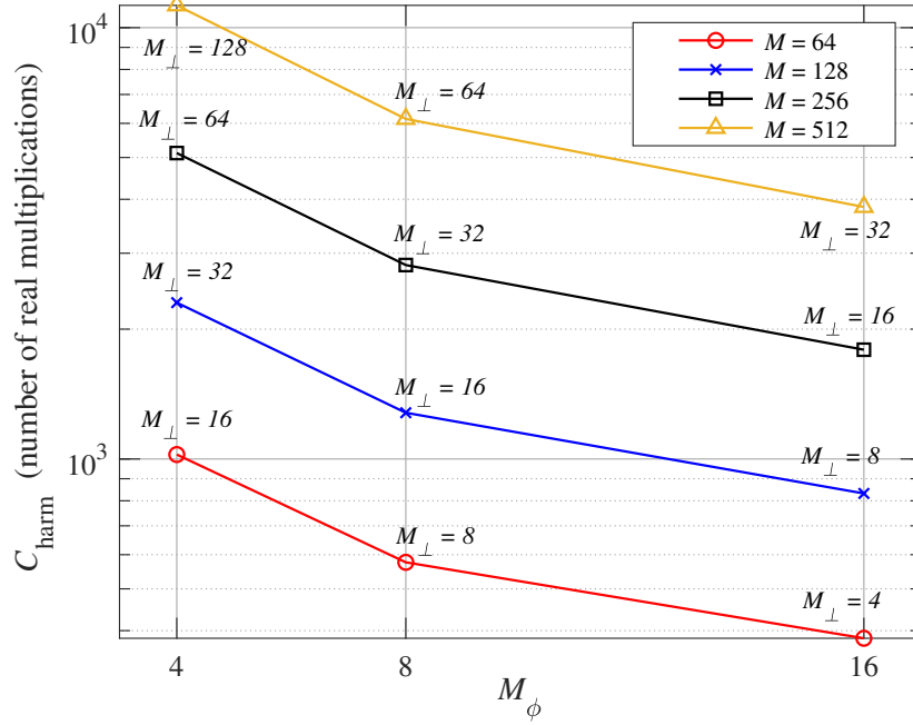
Fig. 3.21 Complexity of 2-tap harmonic receiver for (M_\perp, M_\phi) -AC-FPSK, \mathcal{C}_{\text{harm}} for different modulation orders M = M_\perp \times M_\phi , varying M_\phi and M_\perp .
