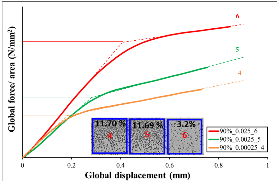
Figure 4-41 Compression results of 90% PPC multilayer samples with change of origin
