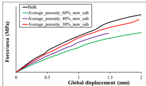
Figure 5-22 3PB simulation results of global displacement vs. global force per unit area with different average porosity (0, 30, 40, and 60%)
