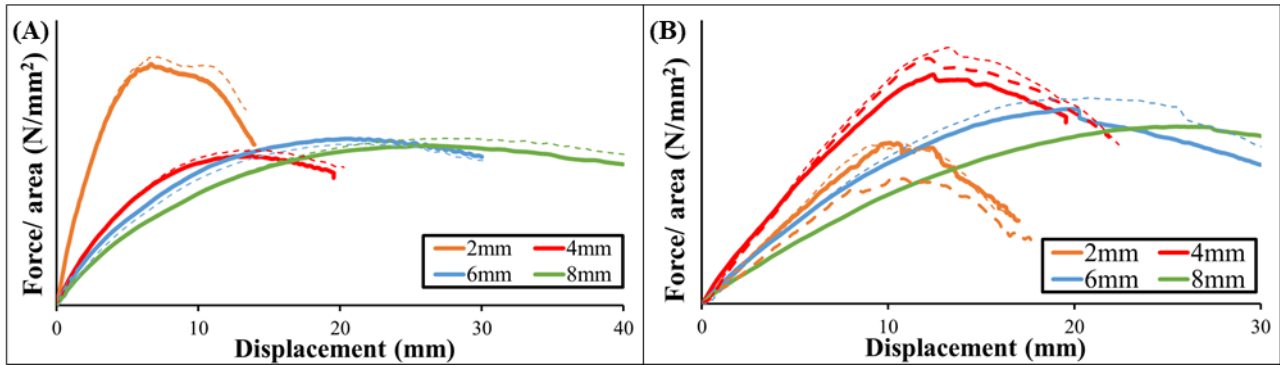
Figure 3-10 (A) 3PB and (B) 4PB test results
