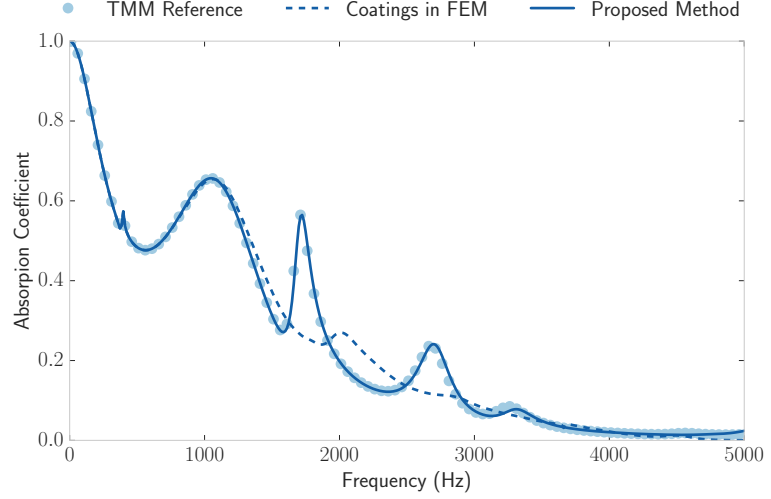
Figure 5.5 – Comparison of the absorption coefficient computed using TMM (circle markers), the proposed method (solid line) or including the coatings in a Finite Element model (dashed line). The number of elements in the core is the same for the two last methods, chosen such as one of them at least complies with the reference.
