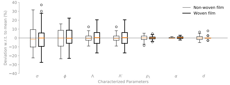
Figure 11 – Spread of the JCA parameters and thickness for both facings. The orange line marks the median, outliers are represented with circles and the box spans between the first and third quartiles. Thin lines correspond to the non-woven facing, thick ones to the woven film. (Color online)
