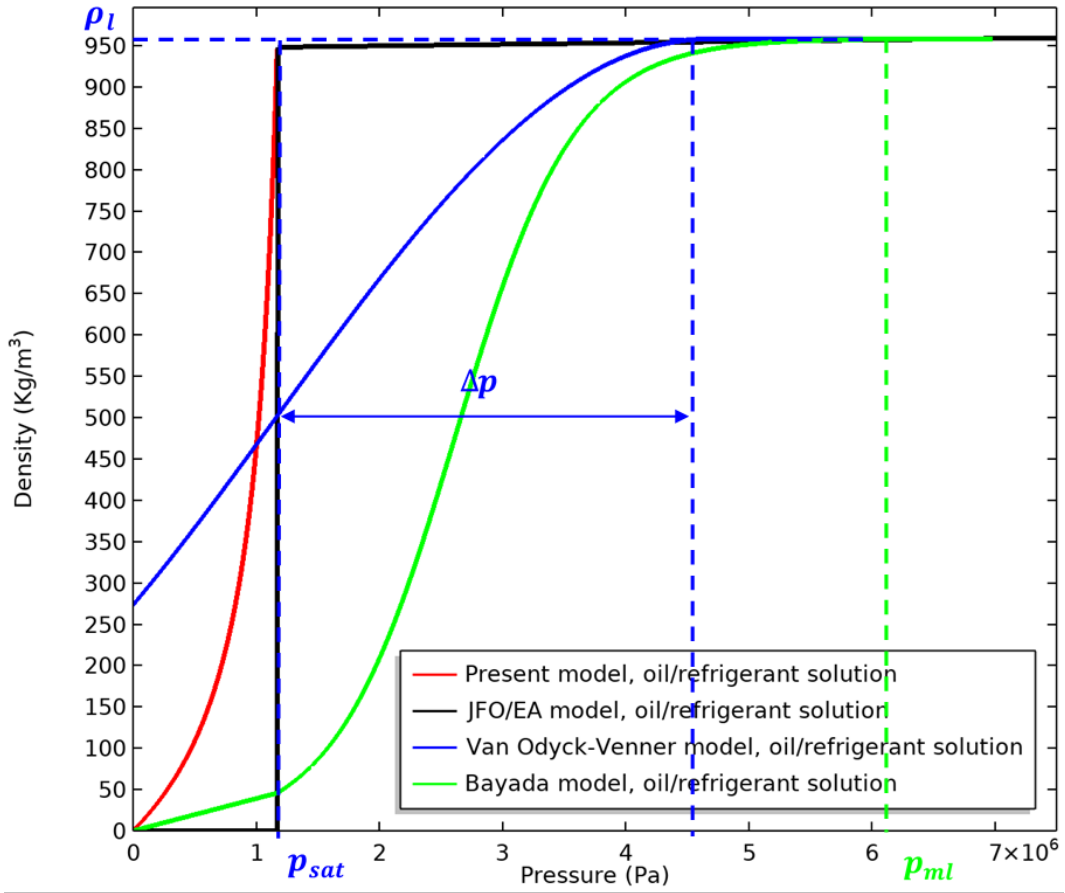
Figure 3.6: The density-pressure relations for the RL68H/R134a solution obtained with different cavitaion models (JFO [43], van Odyck and Venner [132], and Bayada [40]).
