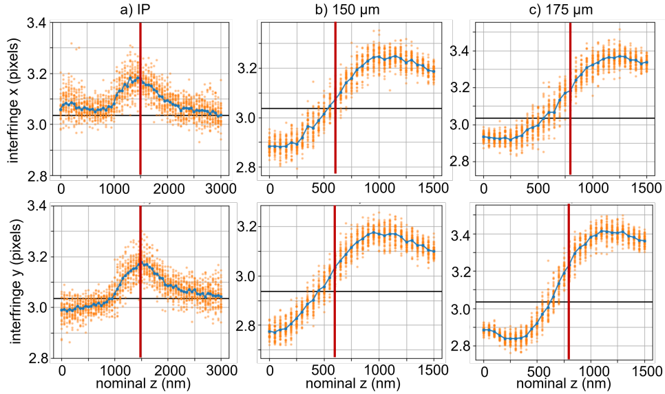
Figure 1.33: Interfringe in x and y as a function of z for different positions of the DG: a) at the IP, b) z_d = 150 \mu\text{m} , and c) z_d = 175 \mu\text{m} from the IP. The red lines indicate where the focus is.
