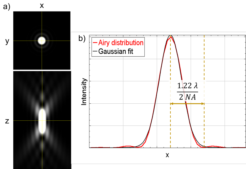
Figure 1.5: a) Simulation of a point spread function of a point-like emitter ( \lambda = 980 nm, similar to SWCNTs) when observed with a microscope of NA = 1.27 . b) A computer-generated image of an Airy disk distribution of intensity in a PSF in comparison to a Gaussian fit.
