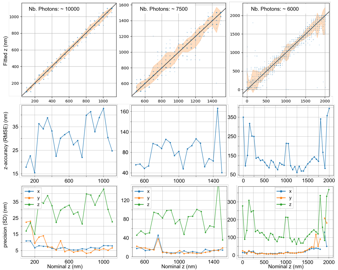
Figure 3.13: z -localization of SWCNTs fixed in the center of the field of view, but different photon budgets.
