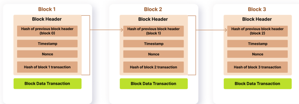
FIGURE 2.2: Blockchain Technology
