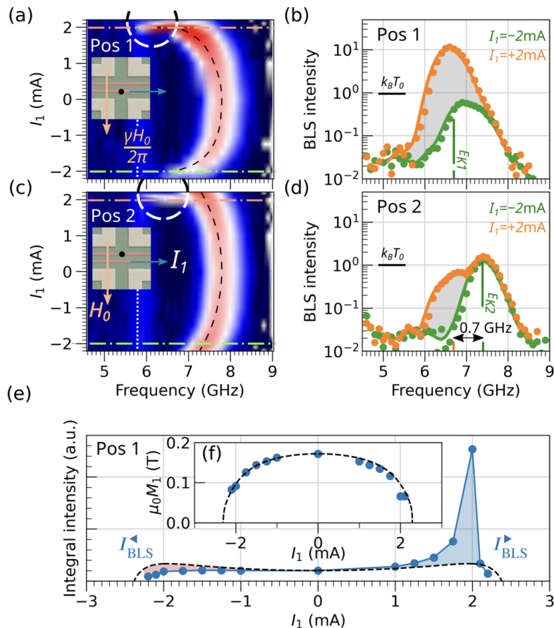
Figure 33: Experimental evidence that the spin diode effect is mainly governed by low-energy magnons. Panels (a) and (c) show the micro-focus Brillouin Light Scattering ( \mu -BLS) spectra as a function of I_1 performed under the two Pt electrodes (see black dot on the insert) at Pos1 (emitter) and Pos2 (collector) for H_x < 0 . Each BLS spectra are renormalized by the amplitude of the Kittel peak at I_1 = 0 . Panels (b) and (d) show two cuts at fixed current I_1 = \pm 2 mA near I_{pk} . The green marker indicates the spectral position of E_K at I_1 = 2 mA. The spectral position of self-localized spin fluctuations, E_{K1} , (see circles) at I_1 = +2 mA (see orange marker) occur clearly below E_{g2} \approx E_{K2} at Pos2 (see green marker). The shift E_{K1} - E_{g2} is about 0.7 GHz. The paramagnetic limit, \gamma H_0 / (2\pi) , is indicated by the yellow vertical dotted line at 5.8 GHz. Panel (e) shows the integrated BLS intensity at Pos1 as a function of I_1 . The solid blue line is a guide for the eyes. The black dashed line shows the expected variation of thermally activated low-energy magnons produced by Joule heating. In echo with Fig. 32, the blue and red shaded areas highlight the variation of magnon emission and absorption with respect to thermal fluctuation. The inset panel (f) shows the evolution of M_1 induced by Joule heating. The blue dots are inferred from the variation of Kittel frequency (dashed parabola in panel (a)). The dashed lines are inferred from SQUID measurements shown in Fig. 31. The data are collected on the YIG_A thin film at T_0 = 300 K using a device with a distance d = 1.0 \mu\text{m} between the two Pt electrodes.
