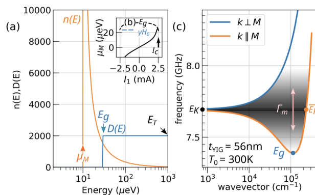
Figure 11: Magnon transport in extended magnetic thin films. (a) In the magnetostatic energy range, magnons behave as a two-dimensional gas, with a step-like density of states, D(E) (blue). The non-equilibrium magnon distribution, n(E) (orange), can be modulated by shifting \mu_M , the magnon chemical potential. (b) In our case, the shift of \mu_M is produced by an electrical current, I_1 , injected in Pt 1 (emitter). (c) Magnon dispersion for different in-plane propagation directions, \theta_k . The plot is shown for the YIG C film at 300 K. The grey shade emphasizes the degeneracy weight of magnons i.e. their propensity to excite parametrically degenerate modes. The black dot indicates E_K , the energy of the Kittel mode ( k \rightarrow 0 ), the blue dot indicates E_g , the minimum of the magnons' band, and the orange dot designates \bar{E}_K , the mode degenerate with E_K with the highest wavevector. The saturation instability described in Fig. 10(b), produces a sharp enhancement of \Gamma_m , the nonlinear coupling between degenerate modes in the energy range E_K \pm (E_K - E_g) . This constrains \mu_M to approach E_g asymptotically at large current as shown in (b).
