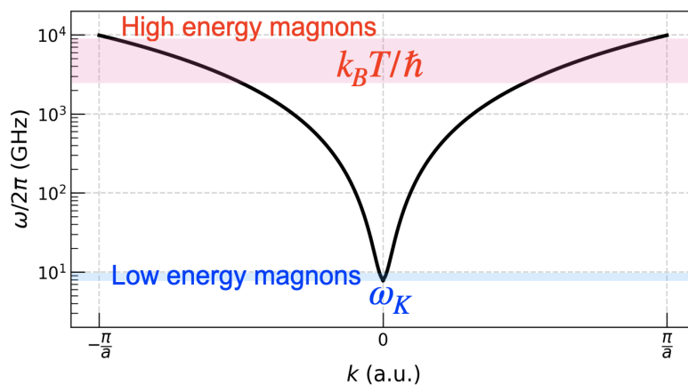
Figure 12: Magnon dispersion relation ranging from GHz to THz energy. \pi/a = 2.55 \times 10^9 rad/m is used from a = 1.2316 nm for YIG.
