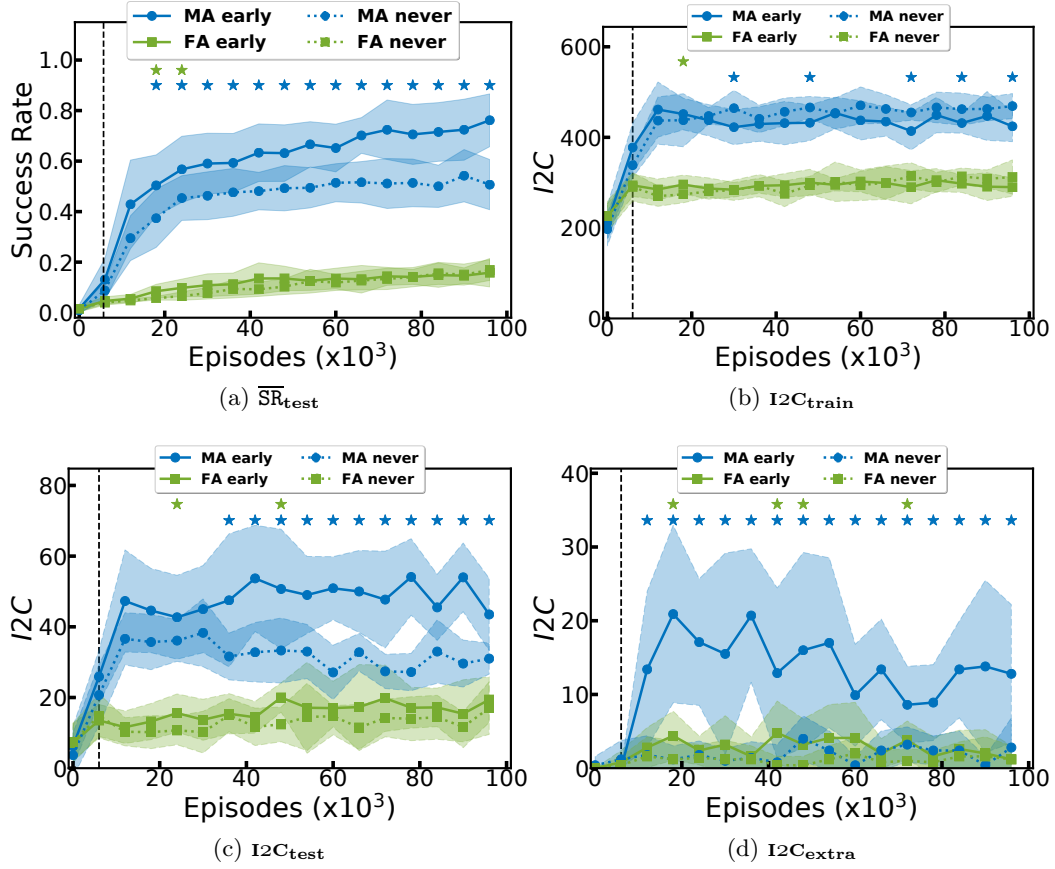
Figure D.8: Policy architecture comparison: (a) \overline{SR} on \mathcal{G}^{test} for the FA and MA architectures when the agent starts imagining goals early (plain, after the black vertical dashed line) or never (dashed). (b, c, d) I2C on interactions from the training, testing and extra sets respectively. Imagination is performed using CGH. Stars indicate significant differences between CGH and the corresponding no imagination baseline.
