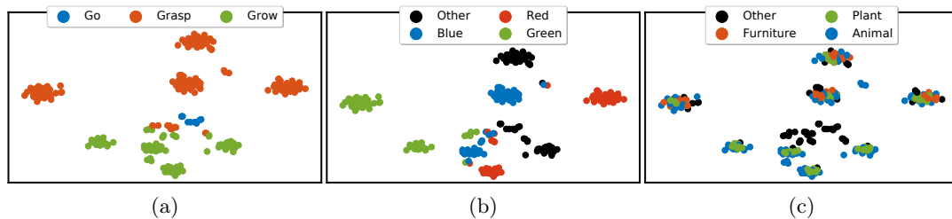
Figure D.9: t-SNE of Goal Embedding. The same t-SNE is presented, with different color codes (a) predicates, (b) colors, (c) object categories.
