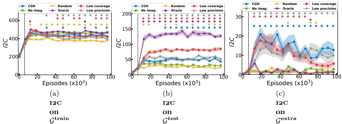
Figure D.6: Exploration metrics for different goal imagination mechanisms: (a) Interesting interaction count ( I2C ) on training set, I2C on testing set, (c) I2C on extra set. Goal imagination starts early (vertical line), except for the no imagination baseline (green). Standard errors of the mean plotted for clarity (as usual, 10 seeds).
