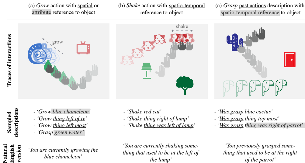
Figure 7.1: Visual summary of the Temporal Playground environment: At each episode (column a, b and c), the actions of an agent (represented by a hand) unfold in the environment and generate a trace of interactions between objects and the agent body. Given such a trace, the environment automatically generates a set of synthetic linguistic descriptions that are true at the end of the trace. In (a) the agent grows an object which is described with spatial (underlined) or attribute (highlighted) reference. In (b) it shakes an object which is described with attribute, spatial or spatio-temporal (underlined) reference. In (c) it has grasped an object (past action underlined) which is described with attribute, spatial or spatio-temporal (highlighted) reference.
