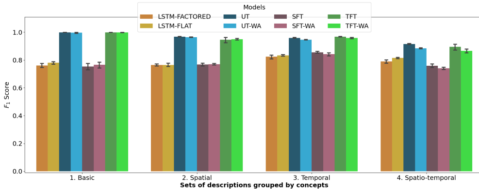
Figure 7.4: F1 scores for all the models on randomly held-out sentences. F_1 is measured on separated sets representing each category of concepts defined in Sec. 7.2.
