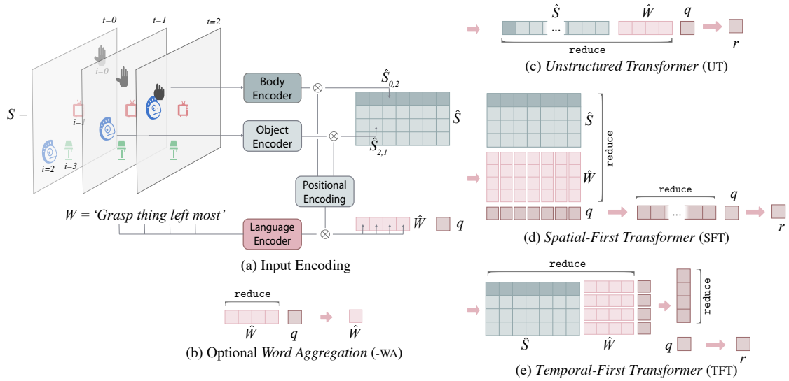
Figure 7.3: Visual summary of the architectures used. We show the details of UT, SFT and TFT respectively in subfigures (c), (d), (e), as well as a schematic illustration of the preprocessing phase (a) and the optional word-aggregation procedure (b).
