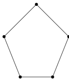
Figure 1.1: An example of a graph depicted in the standard way.
