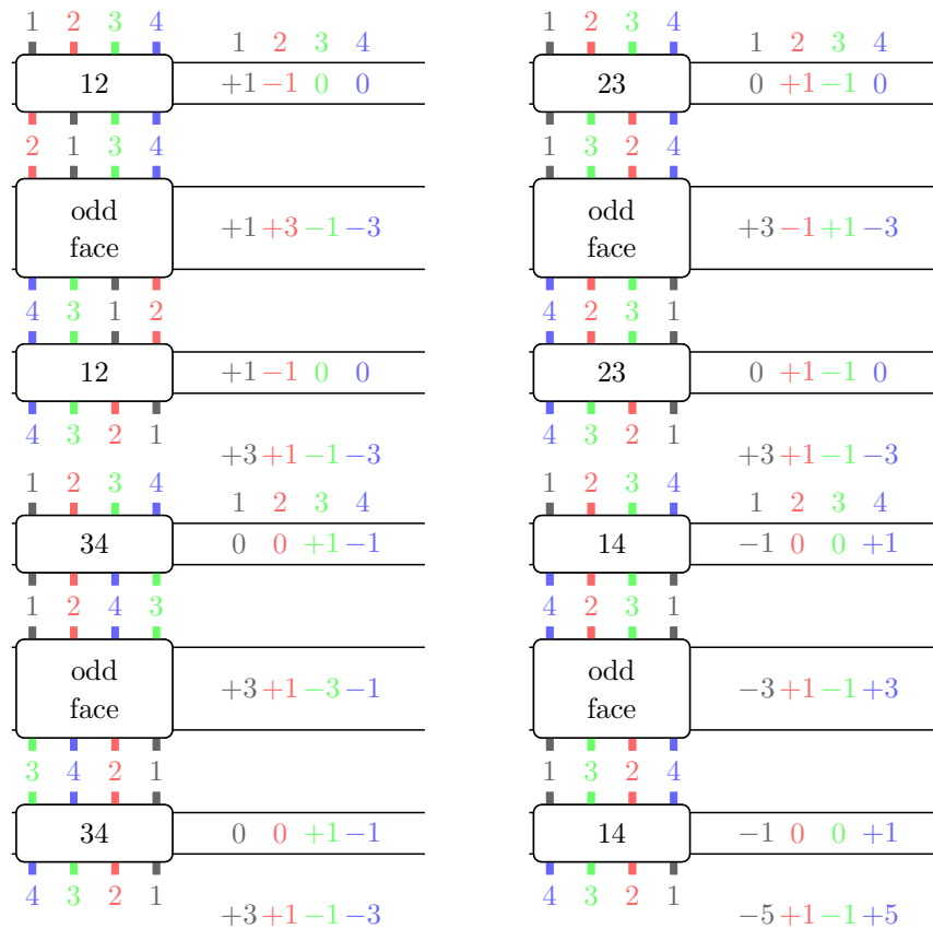
Figure 4.16: When the evolution of an odd face is conjugated, then either it does not change at all, or two of its components gain +8 and -8 respectively. We consider an odd face in such a position that the four colors (read from left to right) evolve by (3, 1, -1, -3) . Observe that these four roles can be played by various quadruples of colors.
