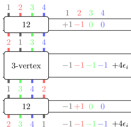
Figure 4.14: The evolution of a lollipop of a vertex v of degree 3 remains invariant even when a swap line the starting point u from v : first, two colors are swapped, then all the colors are rotated, 4\epsilon_i (with i being the color missing at the v ) compensating the rotation, and finally the swapped colors are swapped back.
