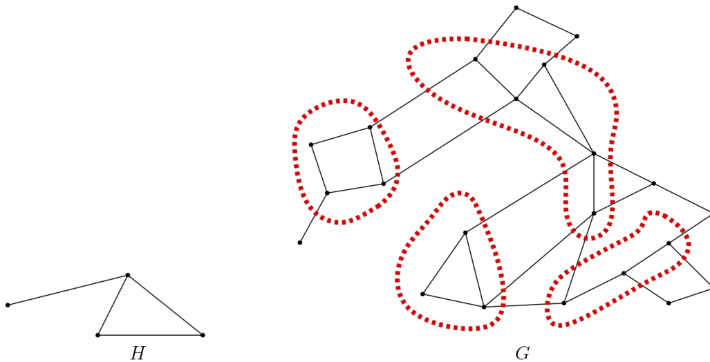
Figure 1.16: By merging the vertices in each red bag in the graph G , we obtain a graph such that H is a subgraph of G : H is a minor of G .
