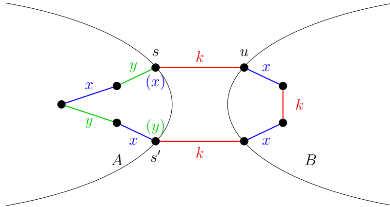
Figure 3.6: If the (x, y) -chain of s' includes s , then G contains an odd cycle.
