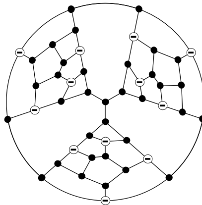
Figure 4.4: The Tutte graph composed of three Tutte fragments.
