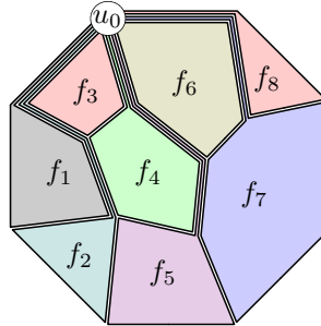
Figure 4.7: The closed walk around a fragment starting and ending at u_0 decomposes into a sequence of lollipops around the faces of the fragment.
