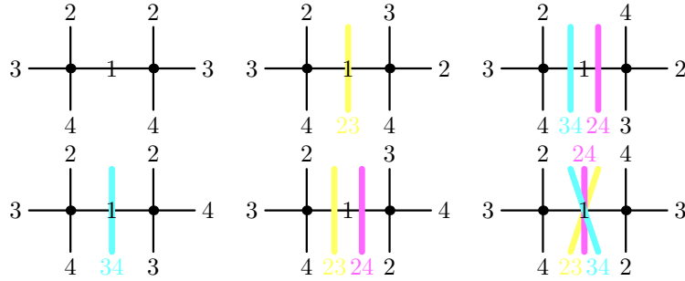
Figure 4.8: For an edge of a given color (here 1), if we fix the three remaining colors at one incident vertex (the left one), there are six possible permutations of these colors at the other incident vertex: Here we list them all and illustrate the corresponding swap-labeling in M(G) , interpreted here as an \Omega -flow in G^* .
