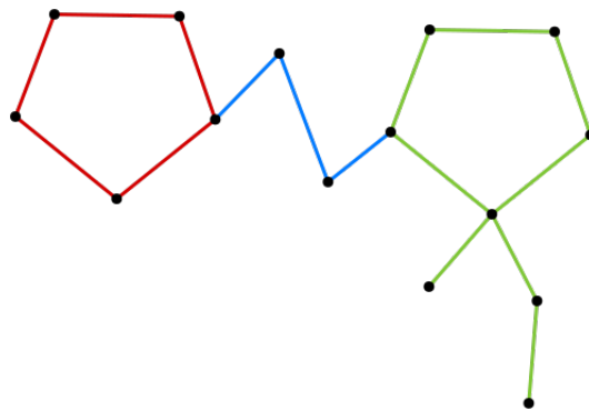
Figure 1.7: Three examples of walks: in red a cycle of length 5, in blue a path of length 3, and in green an open walk of length 8 with a repeated vertex.
