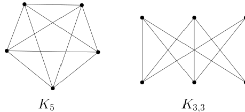
Figure 1.12: The two graphs whose subdivisions are obstruction to planarity.
