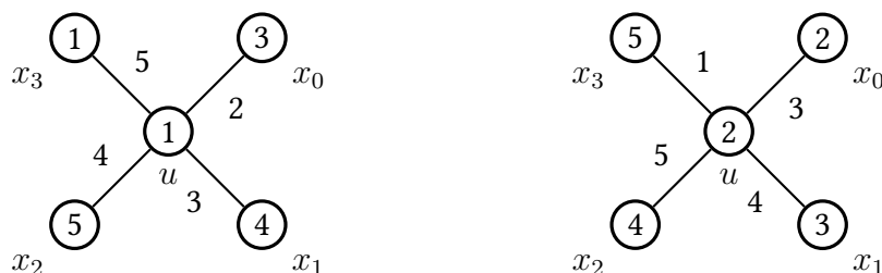
Figure 2.3: Coloring \alpha (left) and X_u^{-1}(\alpha, x_0) (right) when X_u(\alpha, x_0) is a path.
