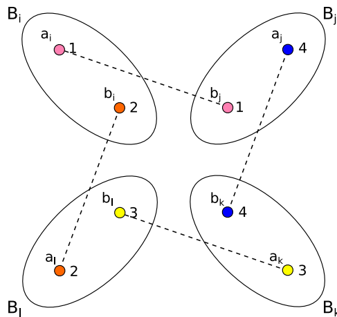
Figure 3.1: A different n -coloring given an appropriate quadruple.
