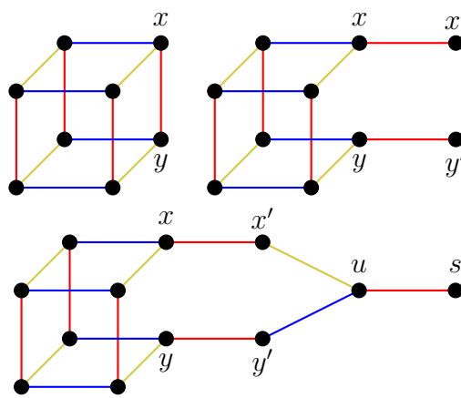
Figure 3.2: The graphs Q_3 , Q_3^+ and H_3 are depicted with possible 3-edge colorings.
