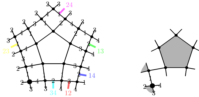
Figure 4.17: An example of a fragment containing a single odd face, with a border coloring (left). A path from the lower-left corner to the odd face, used to calculate the evolution of the face (right). Shaded are the faces that correspond to the orbit of the odd face with respect to \tau along the path. Hence, the evolution of the lollipop of the pentagon is a rotation of (+3, +1, -1, -3) , where the colors play these roles in the order 3, 4, 1, 2.
