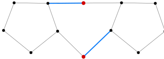
Figure 1.8: The two red vertices form a vertex separator of size 2, and the two blue edges form an edge separator of size 2: this graph is both 2-connected and 2-edge connected.
