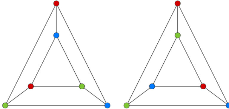
Figure 1.20: Two non equivalent coloring of the triangular prism, each of these colorings is frozen.
