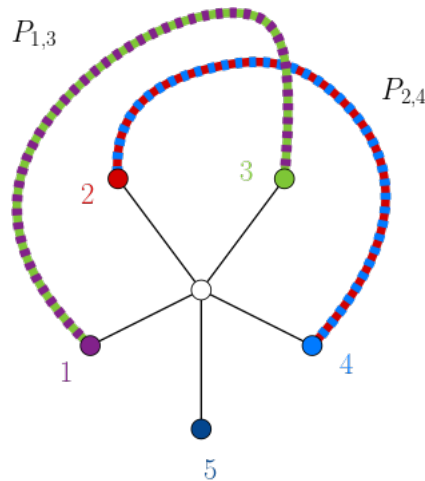
Figure 1.18: P_{1,3} and P_{2,4} cannot share a vertex, so there is an edge crossing; a contradiction since G is planar.
