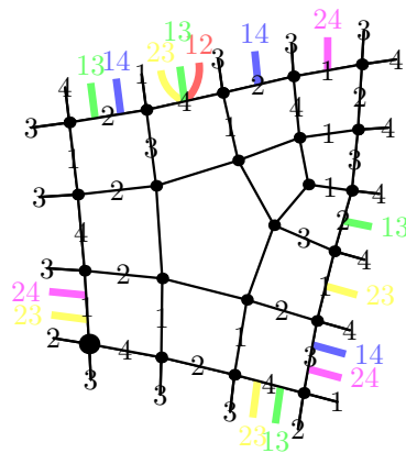
Figure 4.20: Yet another coloring of the border of the fragment from the previous figure. Despite having the same evolution as the previous one, it does not extend to a coloring of the whole fragment.
