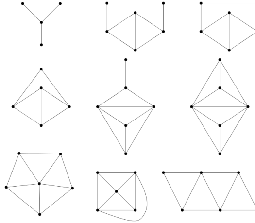
Figure 1.14: The 9 minimum graphs that cannot be induced subgraphs of a line graph.
