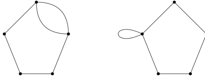
Figure 1.2: On the left-hand side an example of a multigraph with a multiedge, on the right-hand side, an example of a multigraph with a loop .
