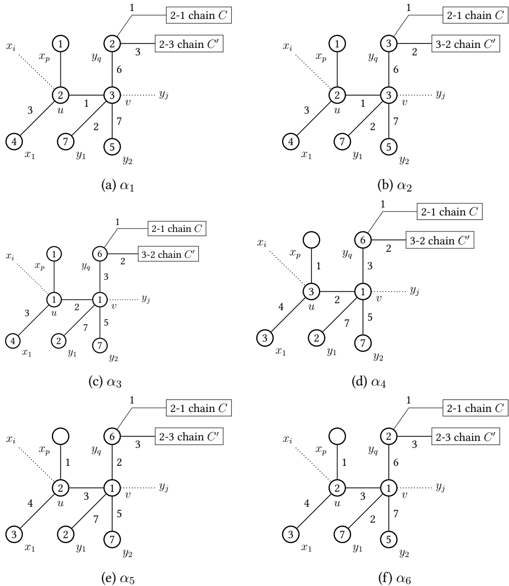
Figure 2.6: Double cycles : illustration of the intermediate colouring in the proof of Lemma 2.2.2.
