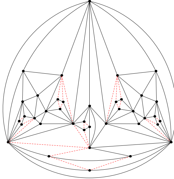
Figure 4.5: The smallest non-4-colorable signed planar graph we have found so far (dashed red lines stand for negative edges).
