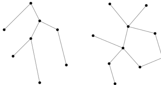
Figure 1.9: On the left-hand side, a tree with 4 leaves; on the right-hand side a graph which is not a tree as it contains a C_5 .
