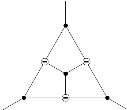
Figure 4.1: An example of a gadget used to replace an odd negative vertex (here k = 3 ).
