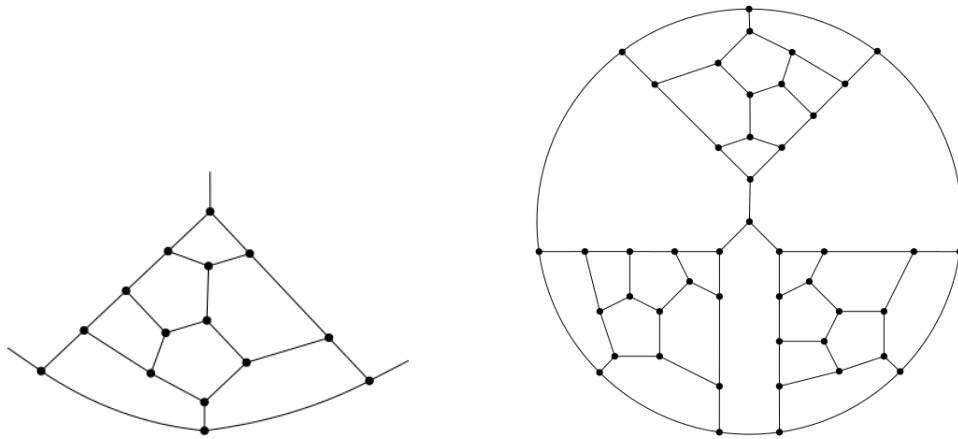
Figure 1.15: The Tutte's fragment and the Tutte's graph.
