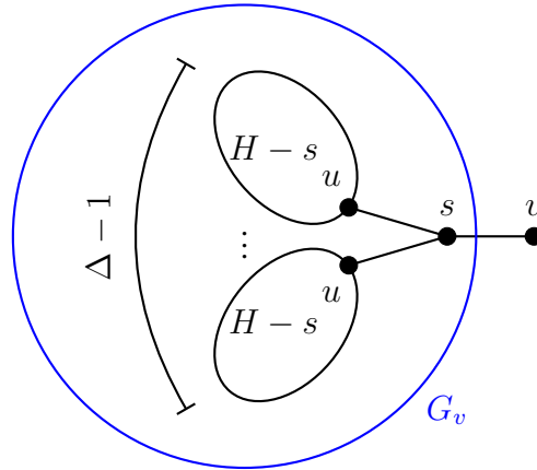
Figure 3.4: We create an instance of the depicted graph for each vertex of G .
