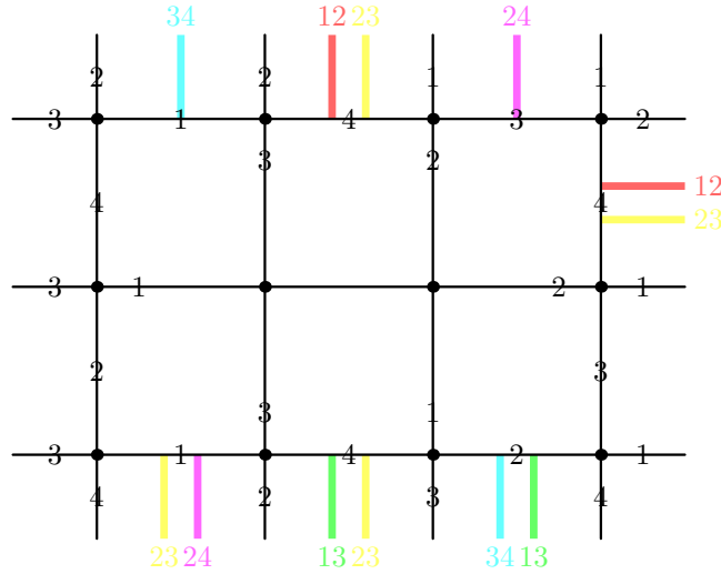
Figure 4.11: Even though the Parity lemma holds, the border coloring does not extend inside the fragment.
