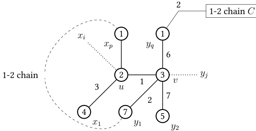
Figure 2.5: Double cycles: Illustration of the beginning of the proof of Lemma 2.2.2: In colouring \alpha , the vertex y_q is in a different component of K(\alpha(uv), m(u)) than u and x_p .
