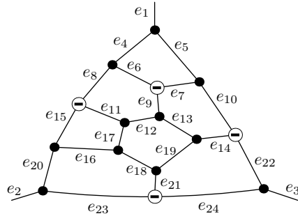
Figure 4.2: A copy of the Tutte fragment with a particular choice of negative vertices.
