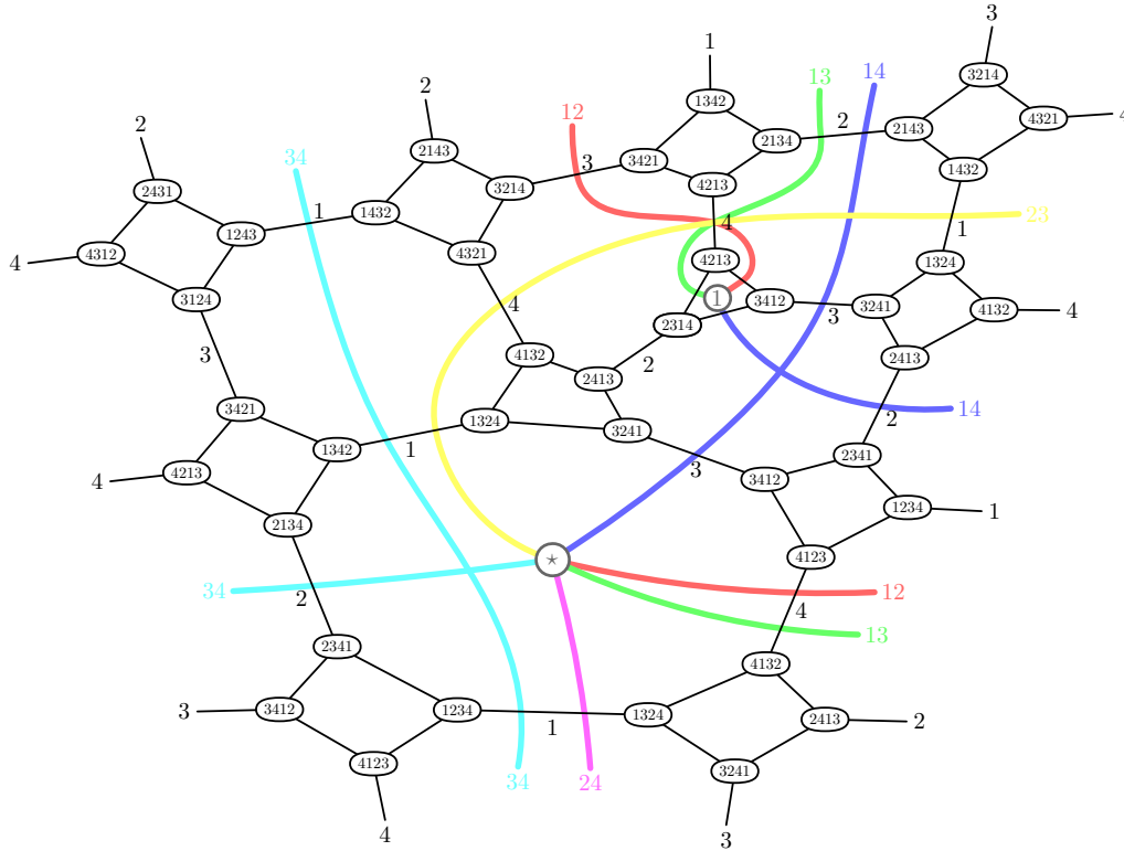
Figure 4.9: An example of the medial graph of a fragment containing one pentagonal face and one vertex of degree 3, with the swap lines interpreted as flow in the dual graph. Observe that the vertex of degree 3 is a source of three swap lines, whereas the face of size 5 is a source of six swap lines.
