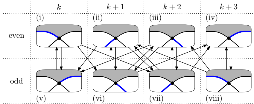
Figure 4.15: A graphical representation of all the possible states of a vertex, with respect to a fixed color (here blue) and the parity of its order taken anticlockwise around a given face (here represented as the grey region). The two rows represent the vertices in even and odd distance respectively, and the values k up to k + 3 represent the evolution of the fixed color. All the possible transitions among the states (when moving from a vertex to the next one) are represented by arrows.
