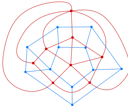
Figure 1.11: The blue graph is a 3-connected planar graph, and the red graph is its dual graph.
