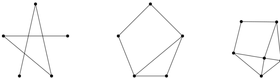
Figure 1.3: In the center, an example of a graph, on the left-hand side, the complement of this graph, and on the right-hand side, the line graph of this graph.
