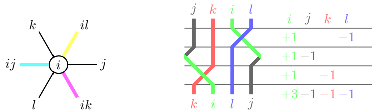
Figure 4.13: A vertex of degree 3 with the missing color i emits three swap lines il , ij , and ik (left). The evolution of a trivial lollipop calculated (right).
