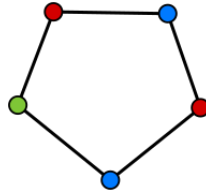
Figure 1.13: A C_5 with a proper vertex-coloring.
