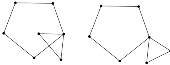
Figure 1.10: On the right-hand side, a planar graph with a planar embedding; on the left-hand side, the same planar graph with a non-planar embedding.
