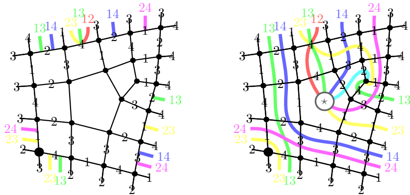
Figure 4.19: Another coloring of the border of the fragment from the previous figure (left). It extends to a coloring of the whole fragment (right).
