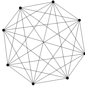
Figure 1.6: The complete graph on 8 vertices.
