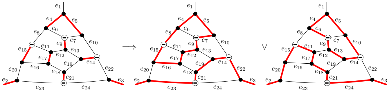
Figure 4.3: In the Tutte fragment with the given position of four negative vertices, for any 2-factor avoiding the edge e_1 there is always at least one cycle containing an odd number of positive vertices.
