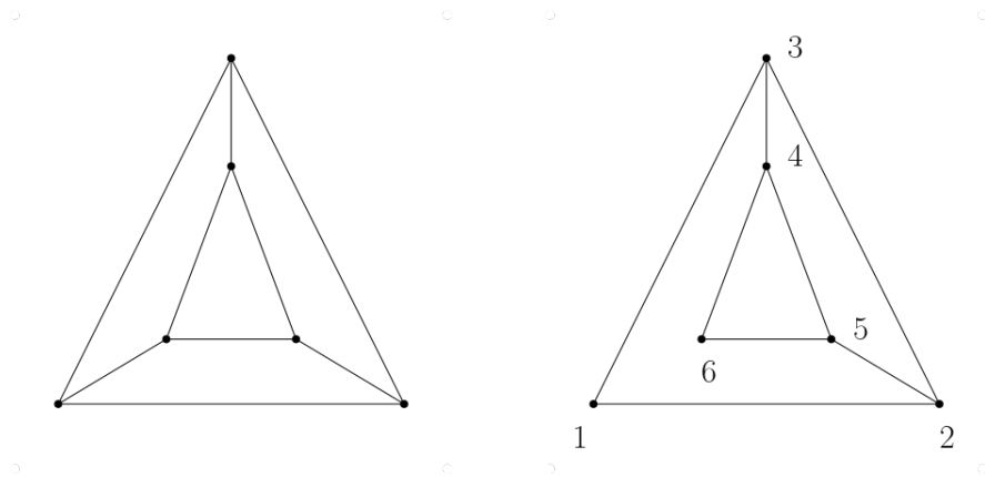
Figure 1.5: On the left-hand side an example of a cubic graph: the triangular prism; on the right-hand side, an example of a 2-degenerate graph with the vertices labeled according to the degeneracy order.
