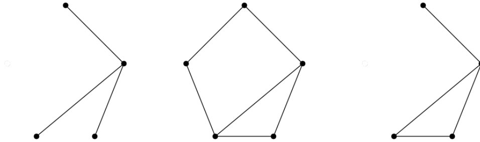
Figure 1.4: In the center, an example of a graph, on the left-hand side, a subgraph of this graph, and on the right-hand side, an induced subgraph of this graph.
