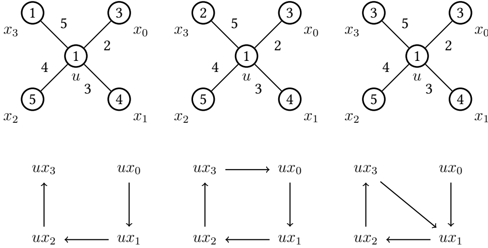
Figure 2.2: From left to right, the three possible scenarios for a sequence X_u(\alpha, x_0) in the digraph D_u(\alpha) : a path, a cycle or a comet. (Vertices are labeled by the missing colors.)
