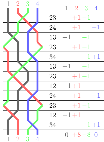
Figure 4.12: An example of a calculation of the evolution of a fragment from Figure 4.11.
