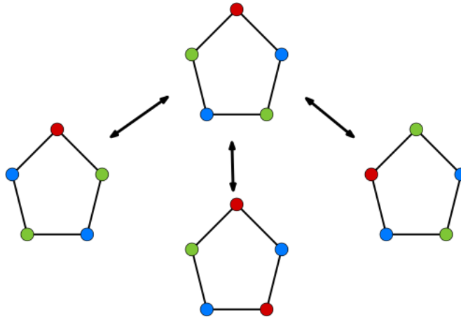
Figure 1.17: Different Kempe swaps applied on a 3-coloring of a C_5 .
