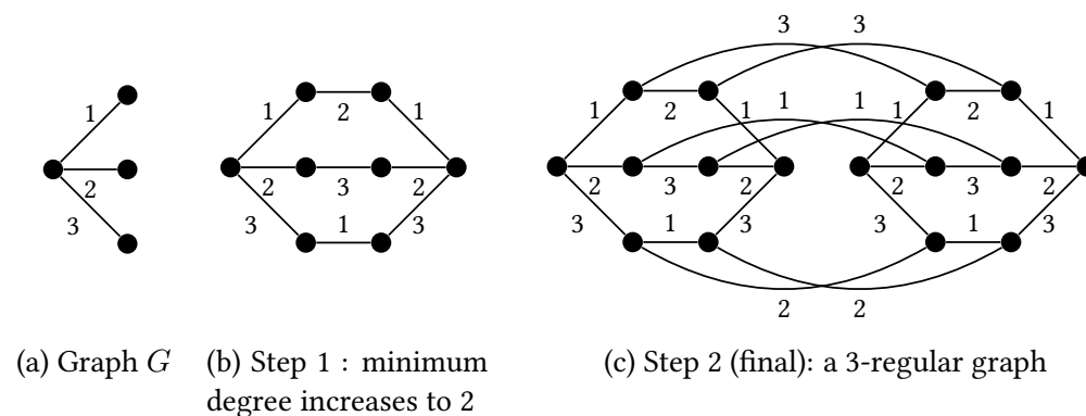
Figure 2.1: Construction of a 3-regular 3-edge colourable graph from a 3-edge colourable graph
