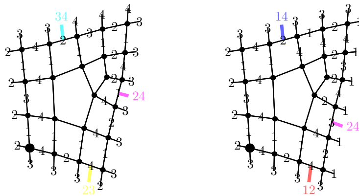
Figure 4.18: An example of a fragment with one odd face and one vertex of degree 3, and two different border colorings. The one on the left is not extendable, whereas the one on the right is. Observe that for both of them the Parity lemma is satisfied.
