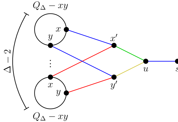
Figure 3.3: The graph H is depicted with a possible edge coloring.
