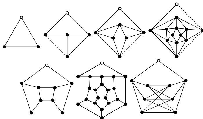
Figure 4.6: Examples of class II graphs of given maximum degree d can be easily obtained by taking a d -regular d -edge-colorable graph and subdividing one edge. For d = 2, 3, 4 , and 5 , planar examples can be found starting with a digon or a platonic solid (first row). For d = 3 and given lower bound on girth (4 or 5), again, platonic solids can do the job; for d = 4 and girth 4, K_{4,4} can be taken for instance (second row).
