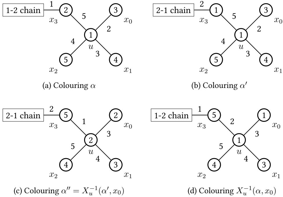
Figure 2.4: Colorings \alpha \rightsquigarrow \alpha' \rightsquigarrow X_u^{-1}(\alpha', x_0) \rightsquigarrow X_u^{-1}(\alpha, x_0) .
