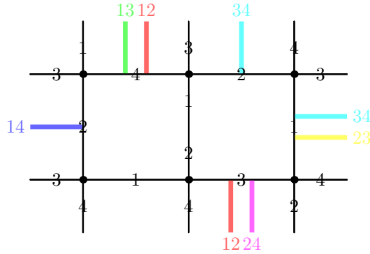
Figure 4.10: The border coloring does not extend, since inside the fragment there are no sources of swap lines, and the border is crossed by an odd number of swap lines of certain types.
