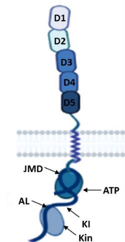
Figure 10 The structure of M-CSF R
