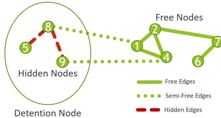
Figure 39: The types of nodes and edges
