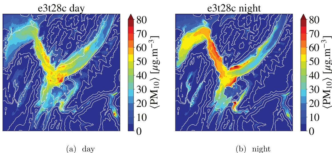
Figure 5.13: Average \text{PM}_{10} levels simulated at 20 m AGL during daytime (a) and nighttime (b) for \mathcal{E}_3 .
