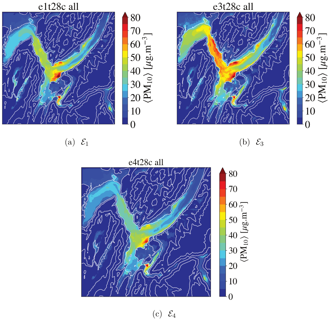
Figure 5.14: Average \text{PM}_{10} levels simulated on the first mass point for \mathcal{E}_1 , \mathcal{E}_3 and \mathcal{E}_4 .
