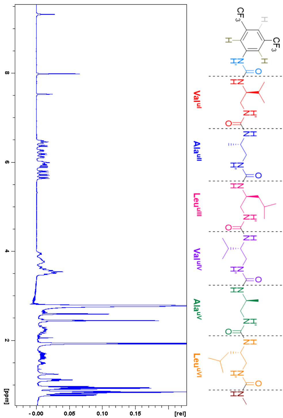
FIGURE A.4. ^1\text{H} -NMR spectrum of 1 in acetonitrile- [d_3] /DMSO- [d_6] (88/12 v/v).
