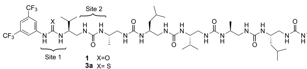
(a) Heptaurea foldamer
