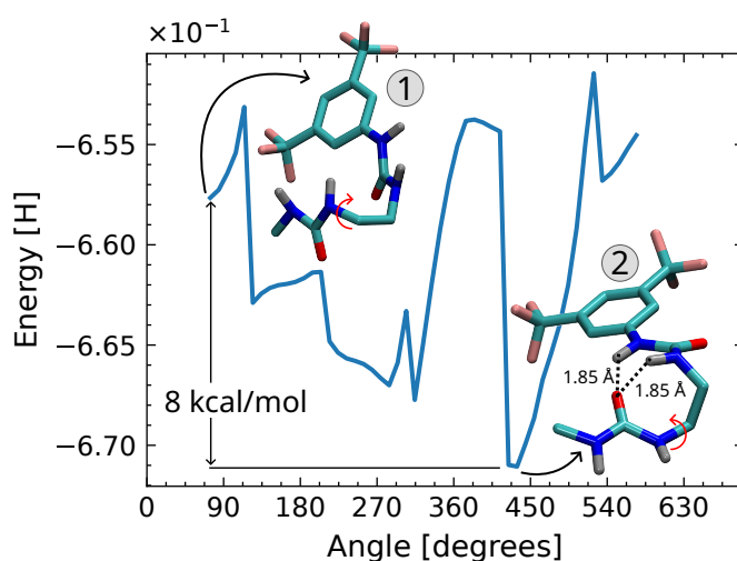
FIGURE B.2. Energetic profile of the coordinate describing the orientation of one urea with respect to the other in the 1-mer. The red arrows show the rotation studied.
