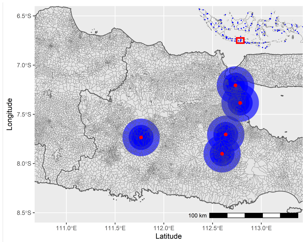
Figure (2.C.5) Geocoded weather stations
