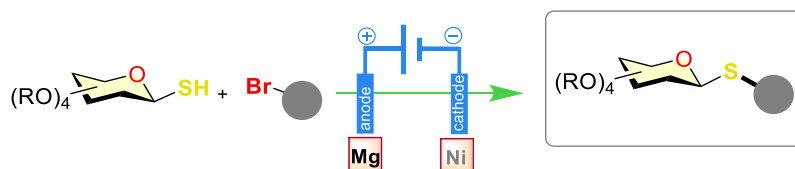
Figure 3. Synthesis of S-glycosides by electrochemistry
