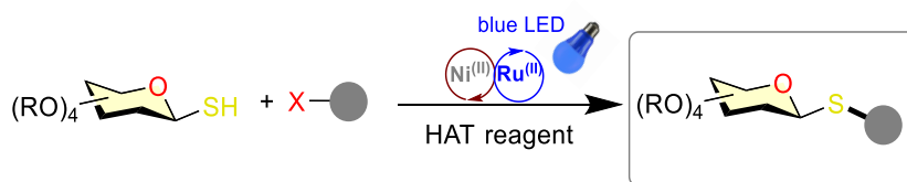
Figure 2. Synthesis of S-glycosides by photoredox reaction
