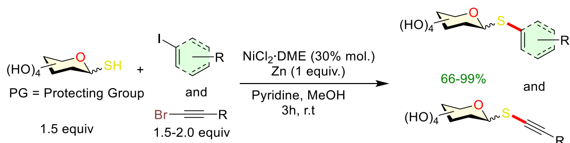
Scheme 8. Coupling of deprotected glycosyl thiols with aryl halides under nickel catalysis.
