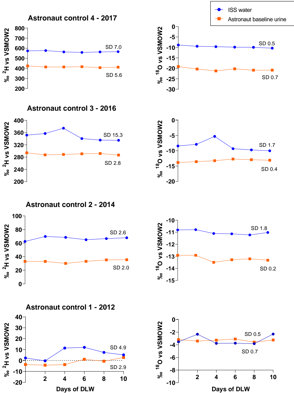
Figure 2: Verification of isotope ( ^{18}\text{O} and ^2\text{H} ) stability for ISS water and control astronaut baseline urine against VSMOW2 IAEA standards during the DLW period measurement.
