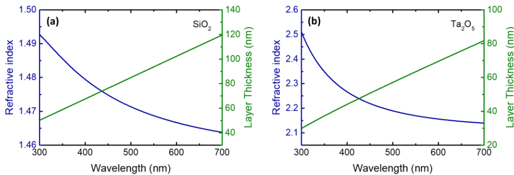
Figure 5.24. Refractive index (blue) and corresponding layer thickness to obtain maximum reflectivity (green) as a function of wavelength for (a) \text{SiO}_2 and (b) \text{Ta}_2\text{O}_5 .
