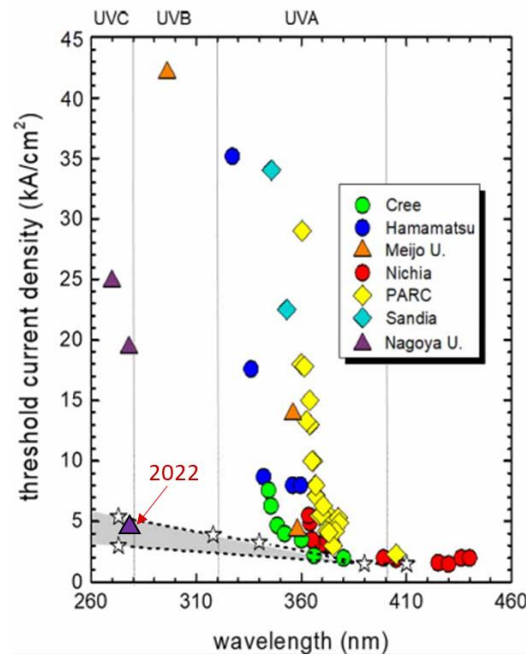
Figure 1.2. Previously published threshold current densities of III-nitride based laser diodes as a function of their emission wavelength. (Reproduced from [3], with data added from [37])
