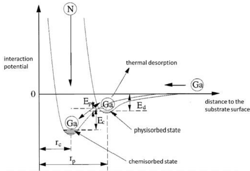
Figure 3.9. Schematic representation of the process during the formation of a GaN layer (taken from [153]).
