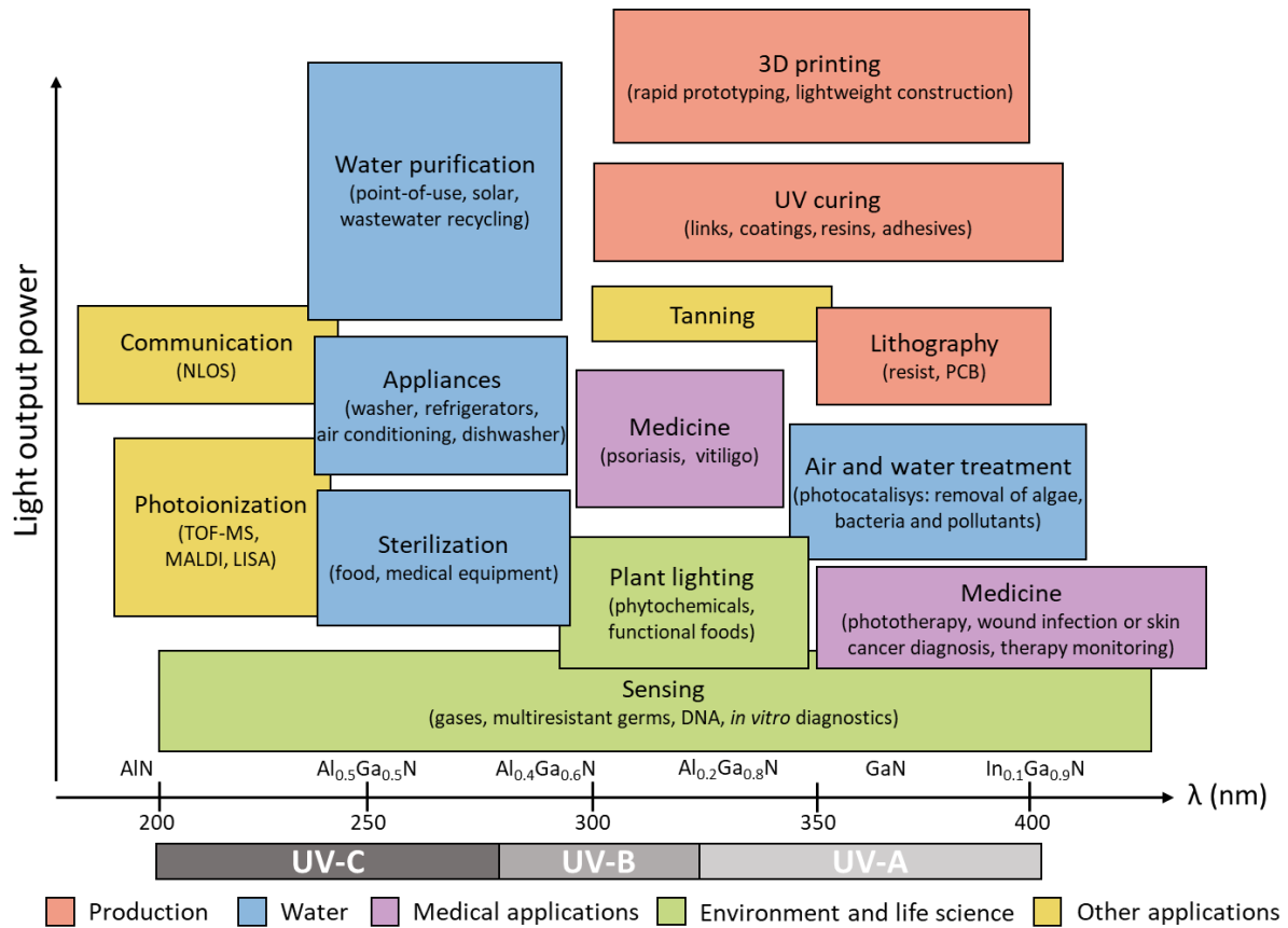
Figure 1.1. Schematic with the main applications of UV emitters. Abbreviations stand for: LISA, Laser Interferometer Space Antenna; MALDI, matrix-assisted laser desorption/ionization; NLOS, non-line-of-sight; PCB, printed circuit boards; TOF-MS, time-of-flight mass spectrometry. (Modified from ref. [2,20])
