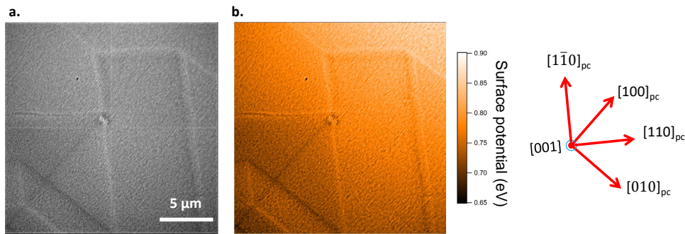
Figure III.17: a. MEM image of the XAS analyzed area. Dark and bright straight lines are domain walls. b. Surface potential map of the analyzed area to identify upward and downward polarized domain walls.
