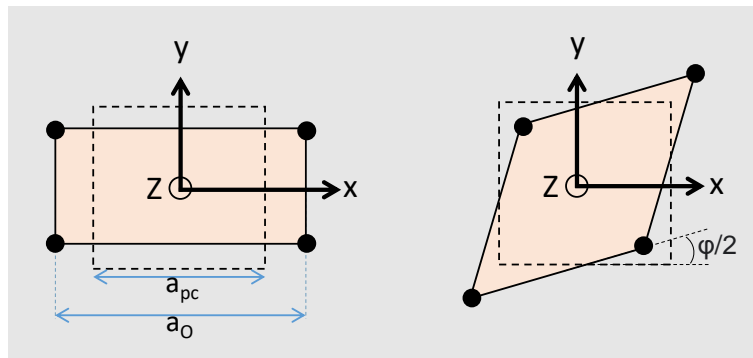
Figure I.8: Two possible transitions between a cubic and an orthorhombic ferroelastic phase for a. a diagonal spontaneous strain term \epsilon_{11} and b. an off-diagonal term \epsilon_{12} . ( x, y, z ) are respectively along the cubic phase directions [001] , [010] , and [001] .
