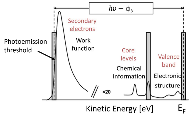
Figure II.4: Typical photoemission spectrum showing the contribution of three types of electrons: secondary electrons and electrons coming from core and valence bands.
