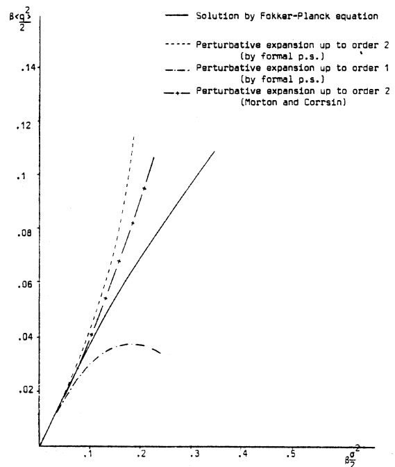
FIG. 2. Second steady-state moment of the solution of the equation \dot{q} + q + q + \beta q^3 = b(t) , \langle b^2(t) \rangle = \sigma^2|t| .
