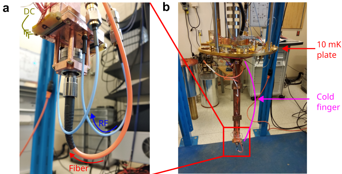
Figure 7.17: Sample holder mounted in a dilution refrigerator. (a) The complete sample holder (PCB and cover with collimator) is mounted to the bottom of a long extended copper-made stick called “cold finger”. The input fiber (red), RF line (blue) and DC lines (olive color) are indicated in the figure. (b) The cold finger is attached to the mix chamber plate of a dilution refrigerator. When it cools down to base temperature, the plate and cold finger should reach 10 mK.
