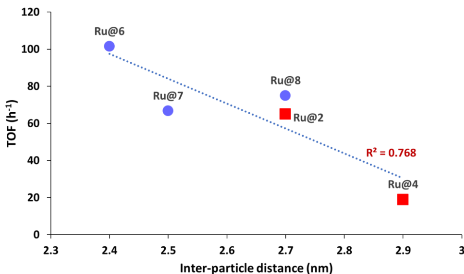
Figure 4.10 Activity as a function of the inter-particle distance in Table 4.6 (blue sphere for amine, and red squares acid ligands), the Ru/ligand ratio in these catalysts is 10/1 (TOF calculated according to the Ru surface content at 1h of reaction).
