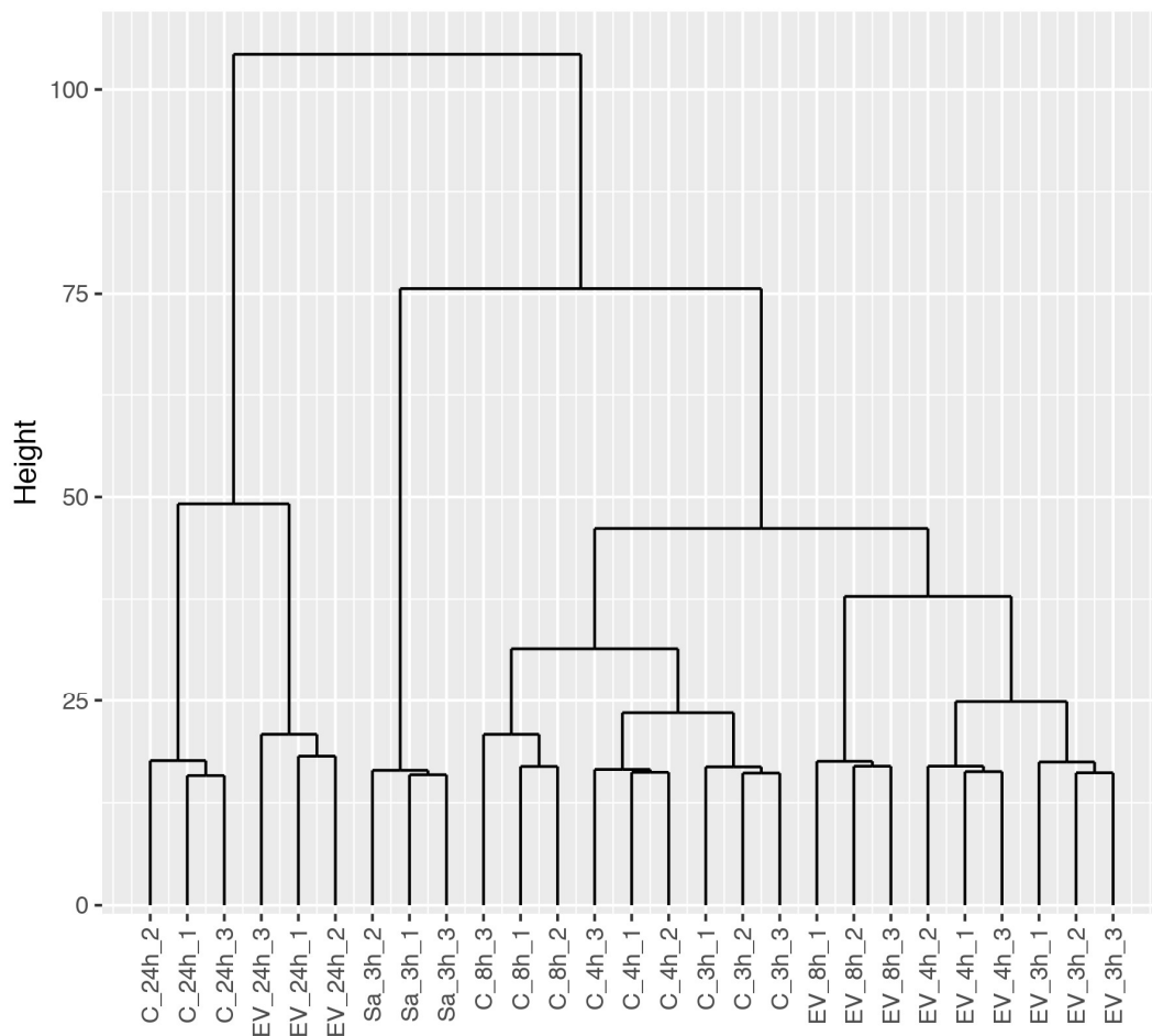
Figure 6.3 Cluster dendrogram.
