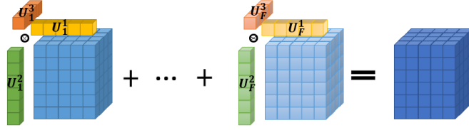
Figure 2.16: Illustration of the CPD. F is the number of outer products formed by mode-1 ( U_i^1 := U_1(:, i) ), mode-2 ( U_i^2 := U_2(:, i) ) and mode-3 ( U_i^3 := U_3(:, i) ) fibers summing up to a tensor with rank F .
