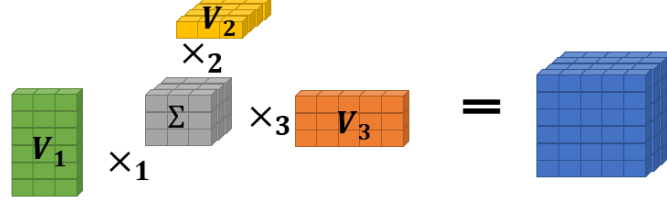
Figure 2.17: Illustration of the exact Tucker decomposition, a generalization of the 2D SVD. A core tensor \Sigma is multiplied along the corresponding modes by base matrices V_1, V_2, V_3 .
