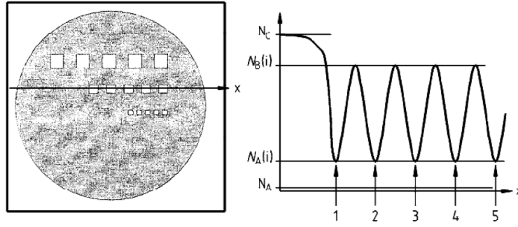
Figure 2.7: Calculation of the spatial resolution from air-material line pair structures. The gray profile is extracted along the structure lines. The contrast factor is calculated from the average difference of its minima (at cut-outs, air), and maxima (material bridges), normalized by the amplitude difference of undisturbed material N_A and undisturbed air N_C . Image source: [14].
