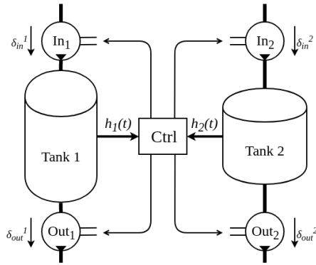
Figure 6.20: One Controllers Two Tanks Configuration
