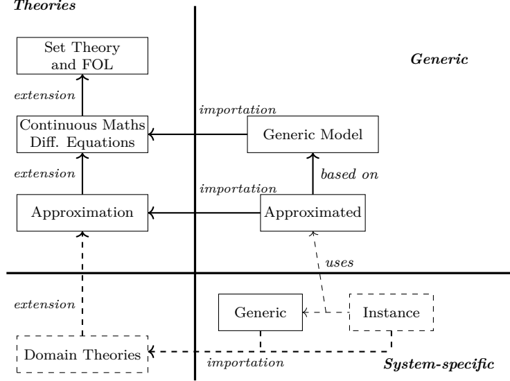
Figure 7.1: Framework – Approximation Pattern
