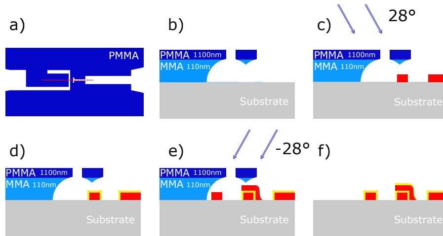
Figure 5.3: Junction deposition with Dolan bridges (a) Top view of the junction mask patterned in a double MAA/PMMA layer by using electron beam lithography. (b) Cross section of a) according the dashed red line. The MMA being more sensitive, undercuts appear below the PMMA layer. (c) First deposition of aluminum with an angle ( 28^\circ ). (d) Oxydation of the aluminum layer (yellow layer). (e) second evaporation with the reverse angle ( -28^\circ ). (f) Lift-off of the resist and oxydation caused by caused by the venting of the sample.
