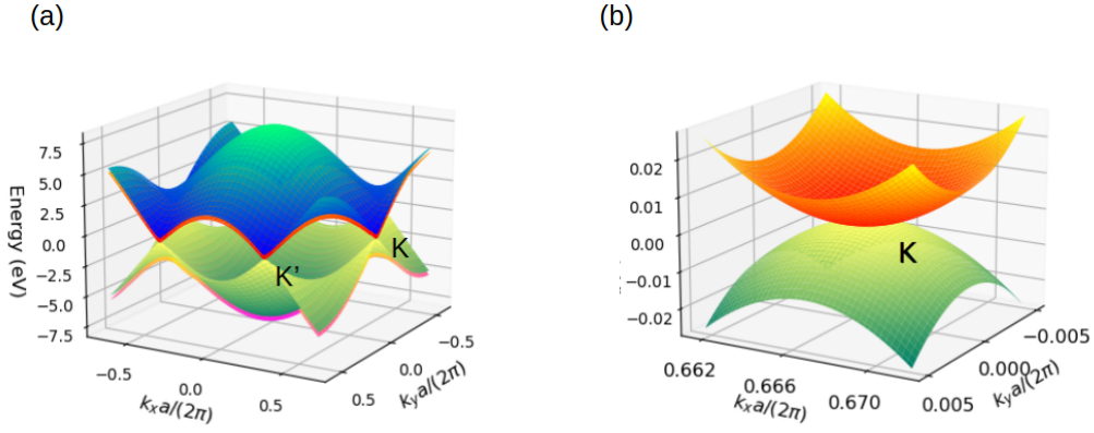
Figure 6.6: (a) Band structure of BLG in the first Brillouin zone. The plot was calculated from the approximate solution (6.15). There are 4 bands: the second lowest band and the third lowest band touch each other at the K-points. (b) In the vicinity of the point K, the dispersion is parabolic.
