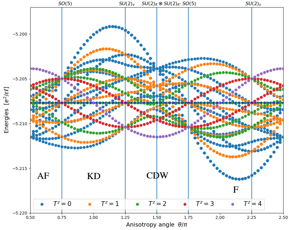
Figure 5.3: Energy levels of the (2/3, 2/3) state on the sphere with N_e = 8, N_\phi = 5 as a function of anisotropy. The unperturbed parent state belongs to the SU(4) irreducible representation (4,4,0,0) . In the SU(4) limit, this irreducible representation is the ground state (lowest-lying state). The energy of the SU(4) parent state is E = -5.20768e^2/\epsilon l (dashed blue horizontal line). The vertical lines mark the high symmetry lines of the anisotropy model we use.
