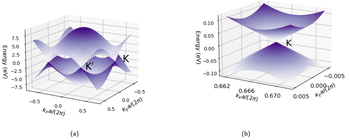
Figure 3.3: (a) The graphene band structure. Here we set \gamma_0 = 2.992 \text{ eV} . The conduction band and valence band touch at the points K and K'. (b) A zoom in the vicinity in the K-point, showing that the band structure is a cone with linear dispersion (Dirac cone).
