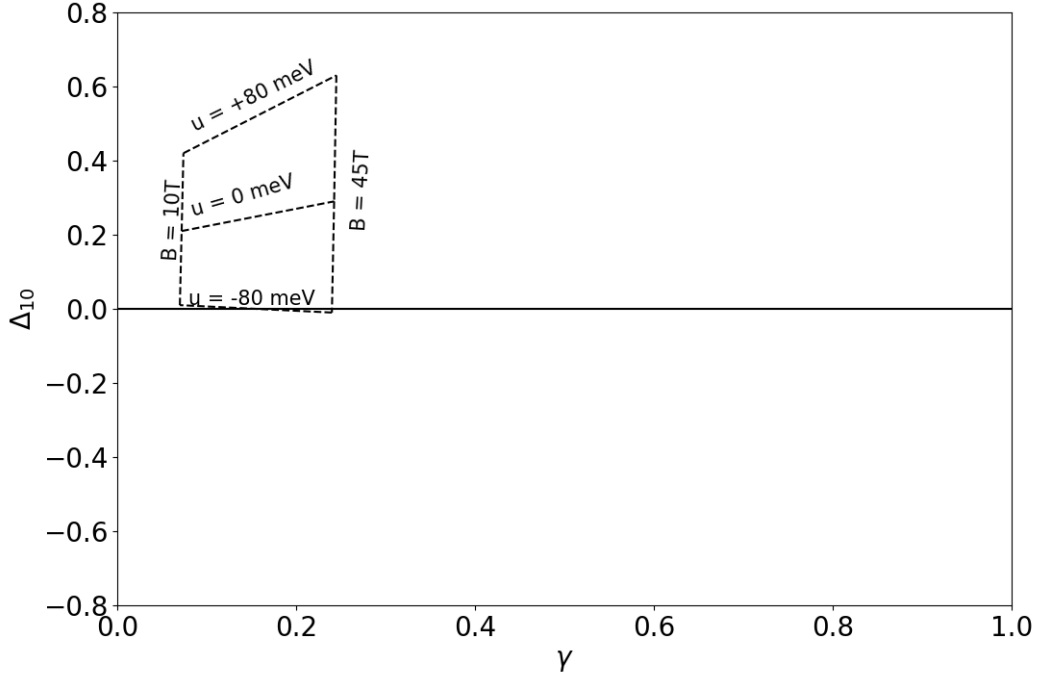
Figure 8.1: The (\gamma, \Delta_{10}) plane. We show the typical values of \gamma and \Delta_{10} accessible during the experiments between the curves corresponding to -80 \text{ meV} \leq u \leq 80 \text{ meV} and 10 \text{ T} \leq B \leq 45 \text{ T} .
