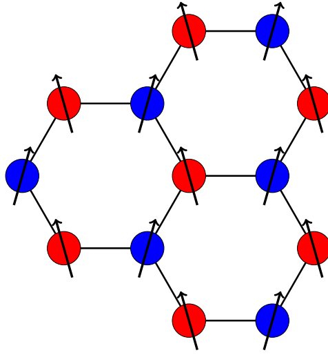
Figure 3.11: Spin polarization of electrons residing in different sublattices in the phase CAF. The spin are canted away from the spin-up direction.
