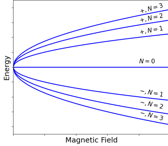
Figure 3.4: Relativistic Landau level spectrum.
