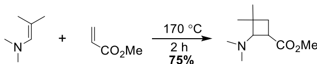
Scheme 47. Preparation of ACBC derivative by thermal method
