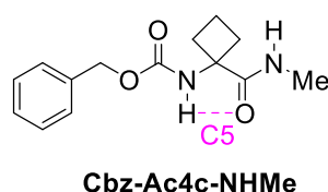
Figure 44. The Cbz-Ac4c-NHMe adopts a minor C5 H-bond conformation in gas phase
