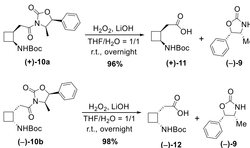
Scheme 16. The cleavage procedure to remove the chiral oxazolidinone (–)- 9
