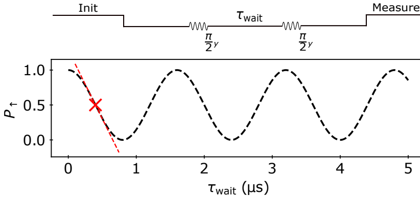
Figure 6.4 – Simulation of Ramsey oscillations for RSS. (Black dashed line) Ramsay oscillations with \Delta f = 1/(4 \tau_{\text{fix}}) where \tau_{\text{fix}} = 400 \text{ ns} (red cross) according to eq. 6.4. The measurement is set up in order to access the linear part of the cosine function (red dashed line is a linear development at the red cross).
