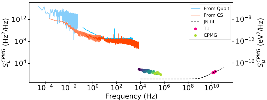
Figure 6.20 – PSD over 14 decades in frequency.
