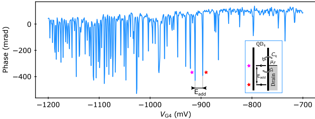
Figure 4.4 – Probing coulomb peaks with drain reflectometry. Main panel : Coulomb peaks of QD4 sensed with drain reflectometry. Inset : schematic showing an orbital level (pink star) of QD4 in resonance with the drain, inducing a tunneling capacitance change.
