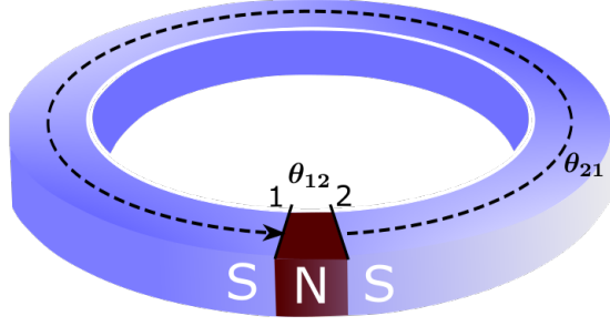
Figure 1.12: A representative sketch of an RF-SQUID. The superconducting ring (blue) is interrupted by a weak link. (dark red) \theta_{21} is the phase drop of the wavefunction in the superconducting part (dashed). \theta_{12} corresponds to the phase drop over the normal part.
