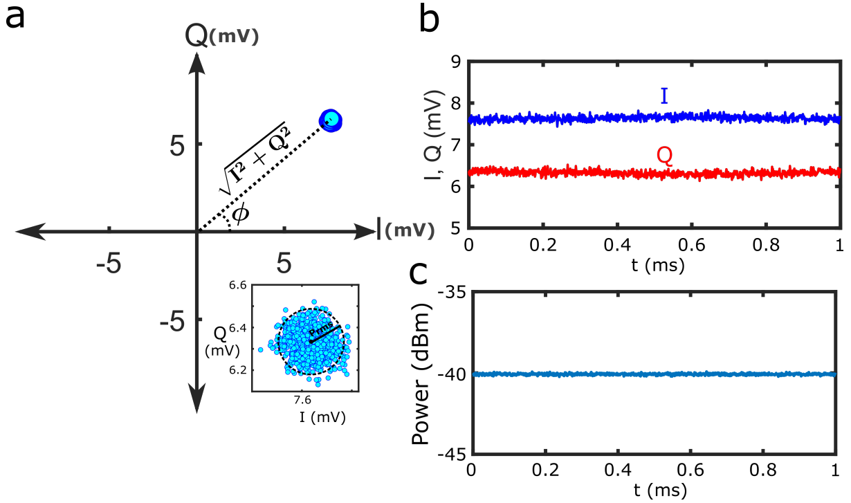
Figure 3.8: A test measurement where the AWG output is directly connected to the VNA input. A sine tone with P = -40 dBm is played for 1 ms. In a , the measured signal is represented in I - Q plane. The inset shows the spread of the datapoints. b . The I - Q components of the same signal as a function of time c . The total power as a function of time
