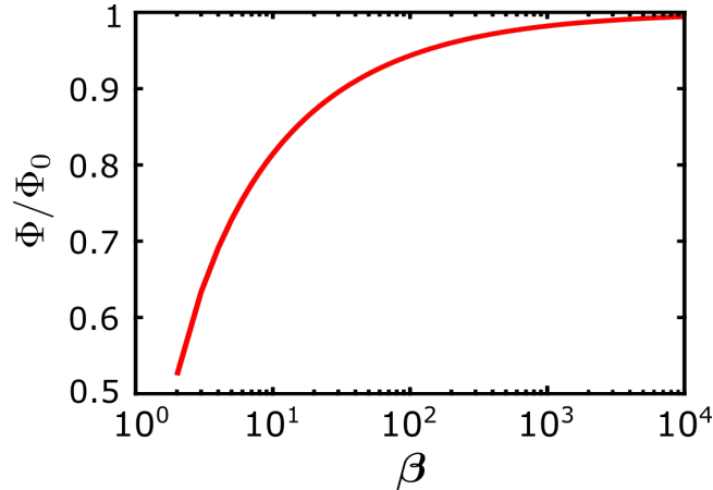
Figure 1.14: The ratio of the flux jump magnitude over \Phi_0 in RF-SQUID as a function of the screening parameter \beta . Note that \Phi \rightarrow \Phi_0 as \beta grows.
