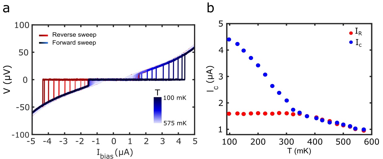
Figure 3.14: a. V - I_{bias} curves of the SNS junction taken between T = 100 mK and T = 575 mK. The forward (reverse) sweeps are marked in the shades of blue (red). b. I_c(T) curve extracted from the data shown in a .
