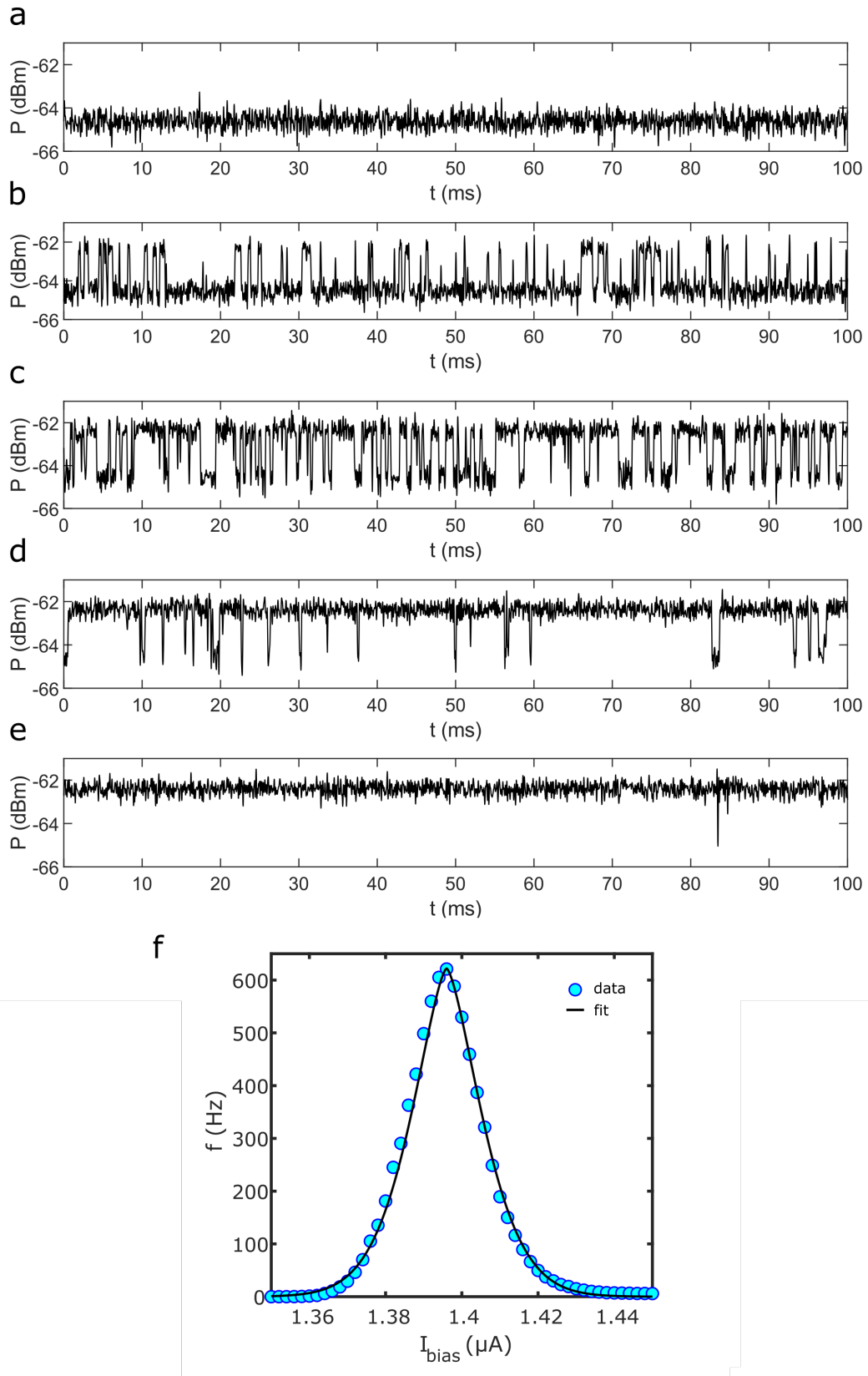
Figure 3.17: The real time measurements taken with f_s = 200 kHz and P_{in} = -100 dBm at a . I_{bias} = 1.35 \mu A b . I_{bias} = 1.39 \mu A c . I_{bias} = 1.40 \mu A d . I_{bias} = 1.41 \mu A e . I_{bias} = 1.45 \mu A f . The extracted switching rates from the real time measurements and the fit with the scaling factor g = 7 .
