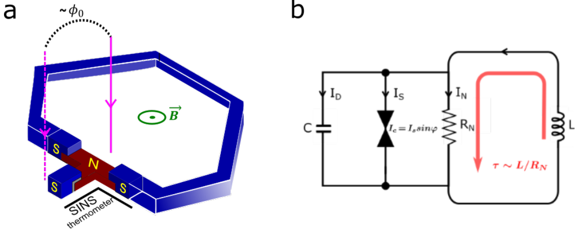
Figure 4.1: a. A sketch of the SQUIPT. The superconducting loop (blue) is interrupted by a normal metal (red). SINS thermometer is formed by the addition of a third superconducting electrode, the oxide layer and the NS lead (black line). A magnetic flux quantum penetrating the loop during a phase slip is depicted with the pink arrows. b The equivalent circuit model of the device. The superconducting loop is represented by its total inductance L . Whenever a phase slips occurs, the difference in internal energy ( \Delta U ) is dissipated on the normal metal (red arrow).
