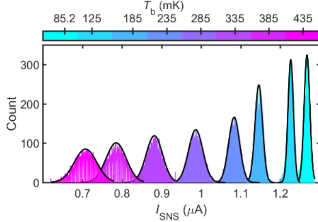
Figure 2.6: Switching current histograms at various bath temperature ( T_{bath} ). Each histogram is fitted with a Gaussian function. The broadening of the histograms at higher T_{bath} originates from the increased thermal noise (taken from [125]).
