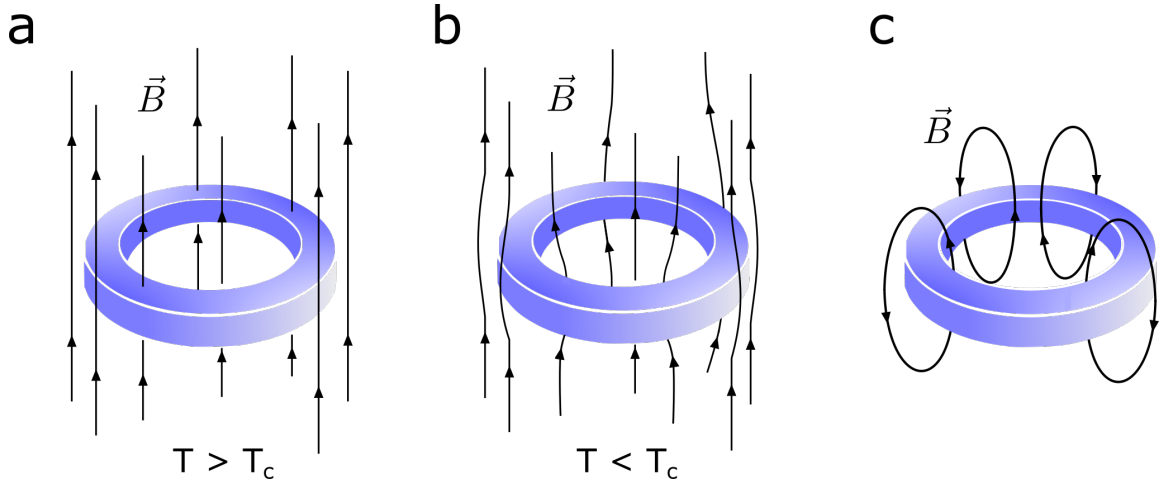
Figure 1.9: A ring in the magnetic field \vec{B} a. in the normal state b. in the superconducting state c. after the external field is removed. (adapted from [76])
