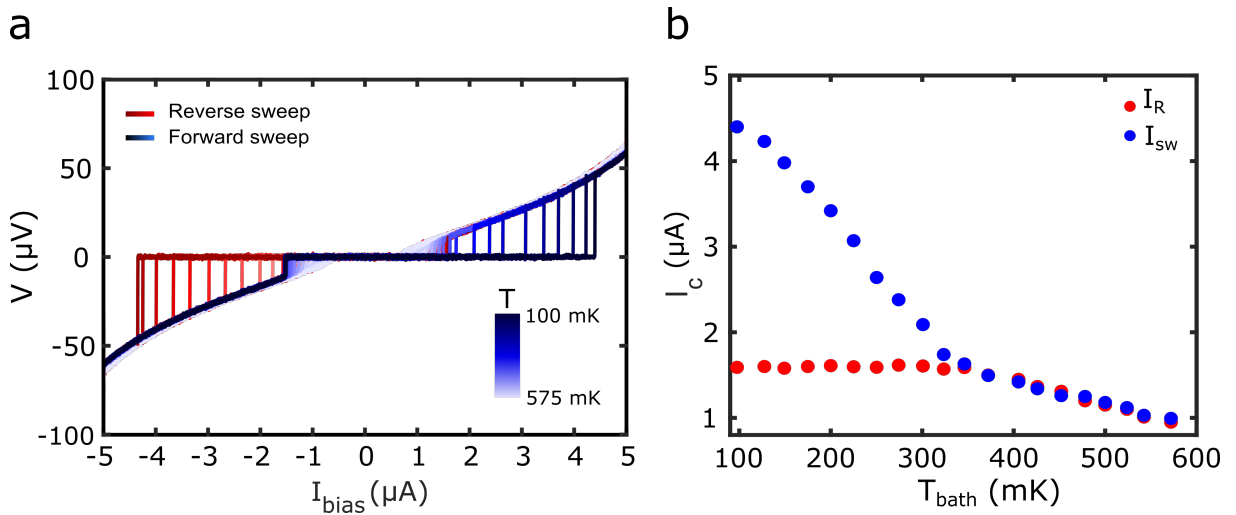
Figure 2.5: a. V(I) curve of an SNS Junction. The forward (reverse) sweep is marked in blue (red). b. I_{sw} and I_R as a function of the bath temperature obtained from a. The hysteresis visible in both subfigures is of thermal origin. Namely, whenever the system switches to the resistive state, Normal island sees an increase in temperature due to the steady-state ohmic heating. As a consequence, the critical current ( I_c ) of the junction decreases to I_c^{steady-state} such that sweeping I_{bias} in the negative direction, the transition N \rightarrow S now occurs when at I_{bias} = I_R = I_c^{steady-state}
