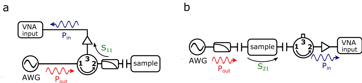
Figure 3.6: The diagrams of typical measurement setups configured for a. reflectometry b. transmittance measurements
