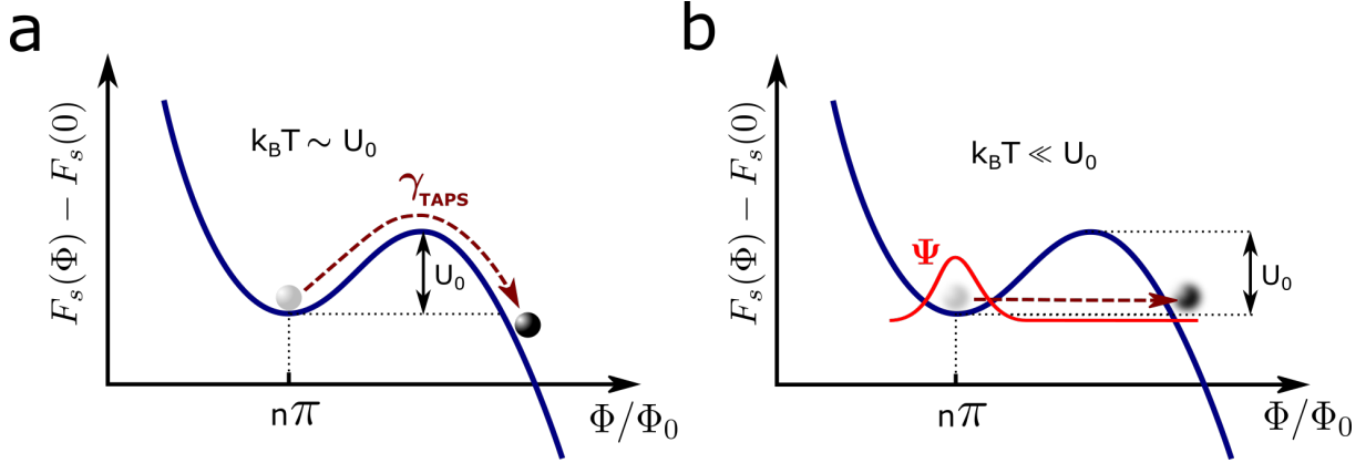
Figure 1.11: a. Thermally activated phase slip. The phase particle surmounts U_0 with a rate \gamma_{TAPS} when k_B T \sim U_0 b. Quantum phase slip. The wavefunction \Psi representing the flux tunnels through the potential barrier. U_0 is the barrier height.
