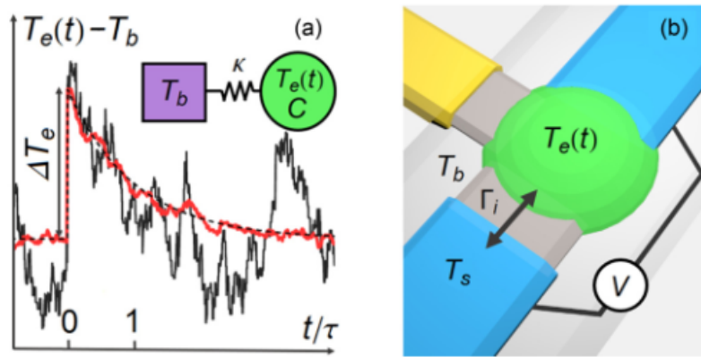
Figure 2.13: a. Monte Carlo simulated time traces of a calorimeter response for a 200\mu\text{eV} impinging energy with T_b = 5\text{ mK} (red) and T_b = 30\text{ mK} (black). [149] b. Schematic of the proposed nanoscale injector-calorimeter setup: A normal metallic island (green) contains a thermalized electron gas, with fluctuating temperature T_e(t) , constituting the absorber. The island is well coupled to an electrically grounded superconductor (upper, blue) acting as a heat mirror. It is further tunnel coupled to another superconductor (lower, blue), kept at a temperature T_s and biased at a voltage V , serving as a particle source with tunable injection rate \Gamma_i(T_s, V) . A thermometer, coupled to the island, is also shown (yellow). (taken from [149])
