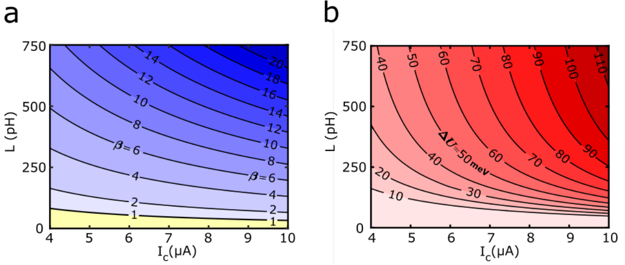
Figure 4.5: a. The 2D contour plot of the screening parameter \beta as a function of the inductance ( L ) and the critical current I_c(T = 0) . The hysteretic regime is shown in gradient blue. The weak screening regime is marked in yellow. b. The 2D contour plot of the change in internal energy \Delta U dissipated on N following a single phase slip with respect to I_c(T = 0) and inductance( L ) .
