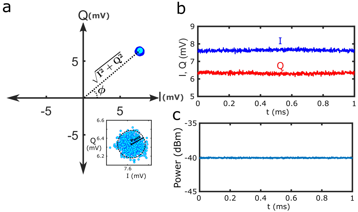
Figure 3.8: A test measurement where the AWG output is directly connected to the VNA input. A sine tone with P = -40 dBm is played for 1 ms. In a. the measured signal is represented in I - Q plane. The inset shows the spread of the datapoints. b. The I - Q components of the same signal as a function of time c. The total power as a function of time
