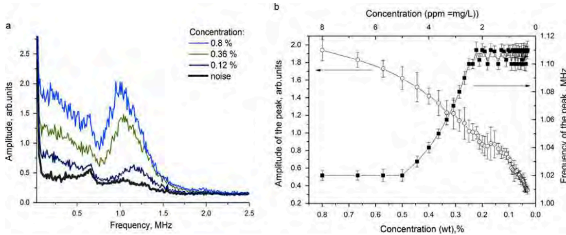
Fig. 26. (a) Computed spectra in experiments with different particle concentrations in water: 0.8%, 0.36% and 0.12%. (b) Experimental dependence, after subtracting the noise, of the amplitude of the spectrum peak (left axis), and the Doppler peak frequency (right axis), on the particle concentration. [37]
