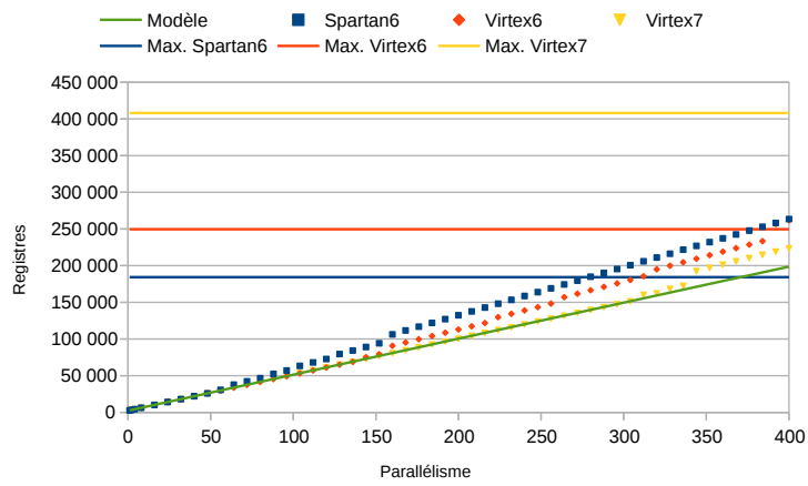
(a) Registres
