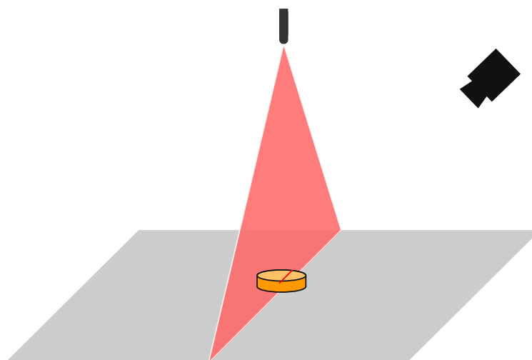
FIGURE 2.1 – Principe de la triangulation laser
