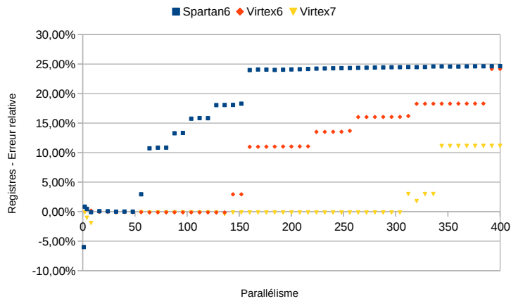
(a) Registres
