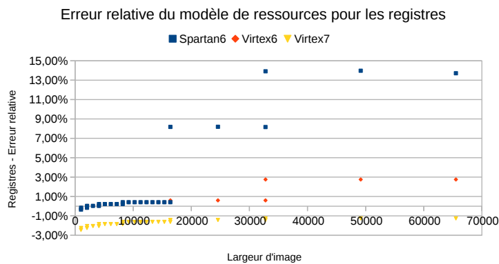
(a) Registres
