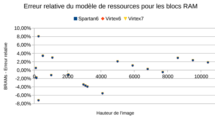
(c) Blocs RAM
