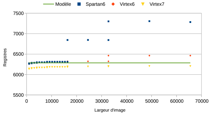
(a) Registres
