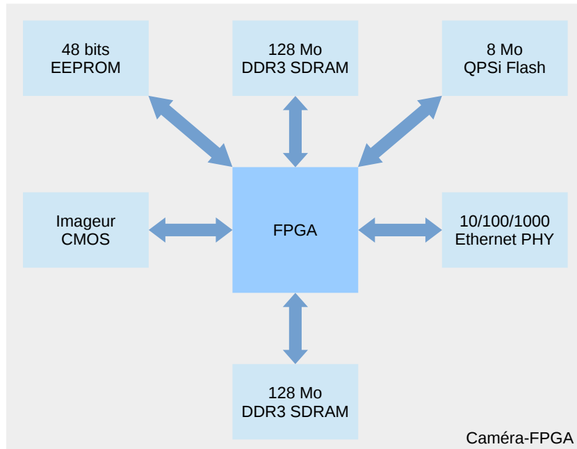
FIGURE 4.1 – Architecture de la caméra-FPGA
