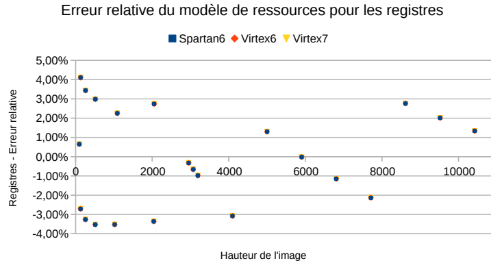
(a) Registres
