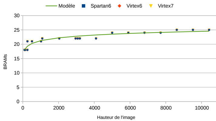
(c) Blocs RAM
