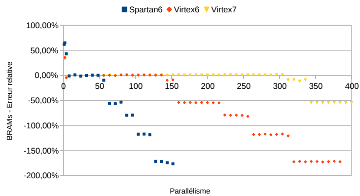
(b) BRAMs
