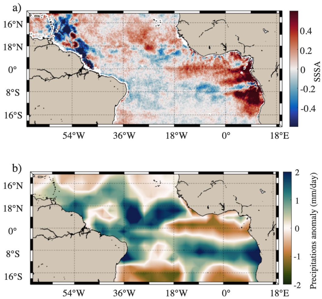
Figure S11. Anomaly to the 2010-2018 climatology for the months of March-April-May-June 2017 in a) SSS, b) precipitations.
