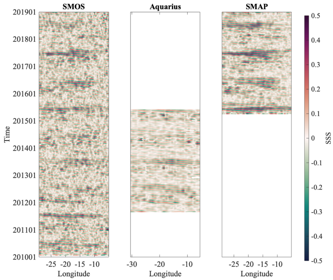
Figure S1. January 2010 to December 2018 Hovmöller diagrams at 1°N of SMOS, Aquarius and SMAP SSSA.
