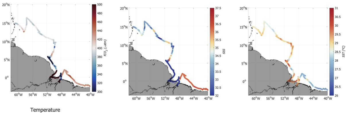
Figure 3.5: From left to right, Tara’s in-situ near surface measurements of fCO 2 , salinity and temperature.
