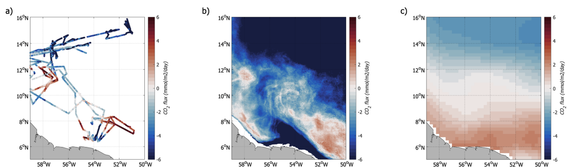
Figure 7.10: a) Air-sea \text{CO}_2 flux measured in Jan-Feb 2020 during the EUREC 4 A-OA/ATOMIC cruise. b) Air-sea \text{CO}_2 flux reconstructed over February 2020. c) February climatology of the air-sea \text{CO}_2 flux over 1998-2015 (Landschützer et al., 2020).
