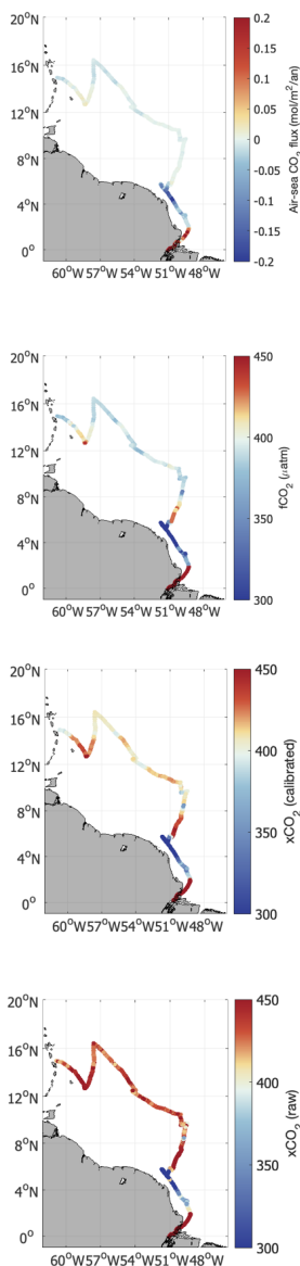
Figure 3.8: From top to bottom, final air-sea CO 2 flux, sea water fugacity of CO 2 , calibrated sea water xCO 2 , and raw sea water xCO 2 from Tara leg 5.
