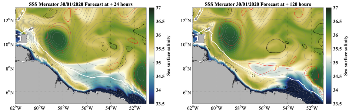
Figure 6.4: Mercator PSY2V4 model SSS (color) and sea level (gray contours) forecast and eddy detection made on the January 30, 2020 for January 31, 2020 (left) and February 4, 2020 (right). The eddy detection is shown by dashed contours (red for anticyclones and black for cyclones; Laxenaire et al., 2018). The shelf break is represented by the 100-m bathymetry contour (white line).
