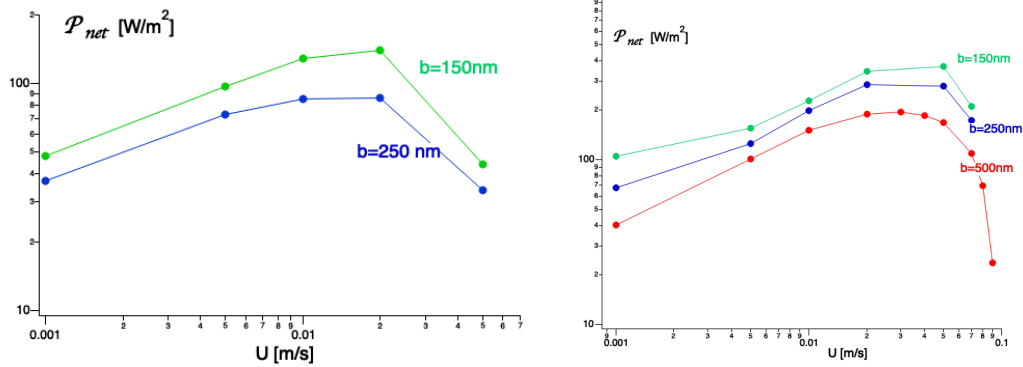
Figure 4.7: Left: Power density generated from the 3D simulation of the Elemental Exchanger plotted against microchannel convection velocity for microchannel width b = 250, 150\text{nm} . The velocity profile for the exchanger is shown in fig. 4.6. Right: Same plot for an exchanger with a velocity source in the middle of the microchannel, instead of the edge. It can be seen that is configuration of the exchanger produces approximated 2.5 times more power compared to the other configuration.
