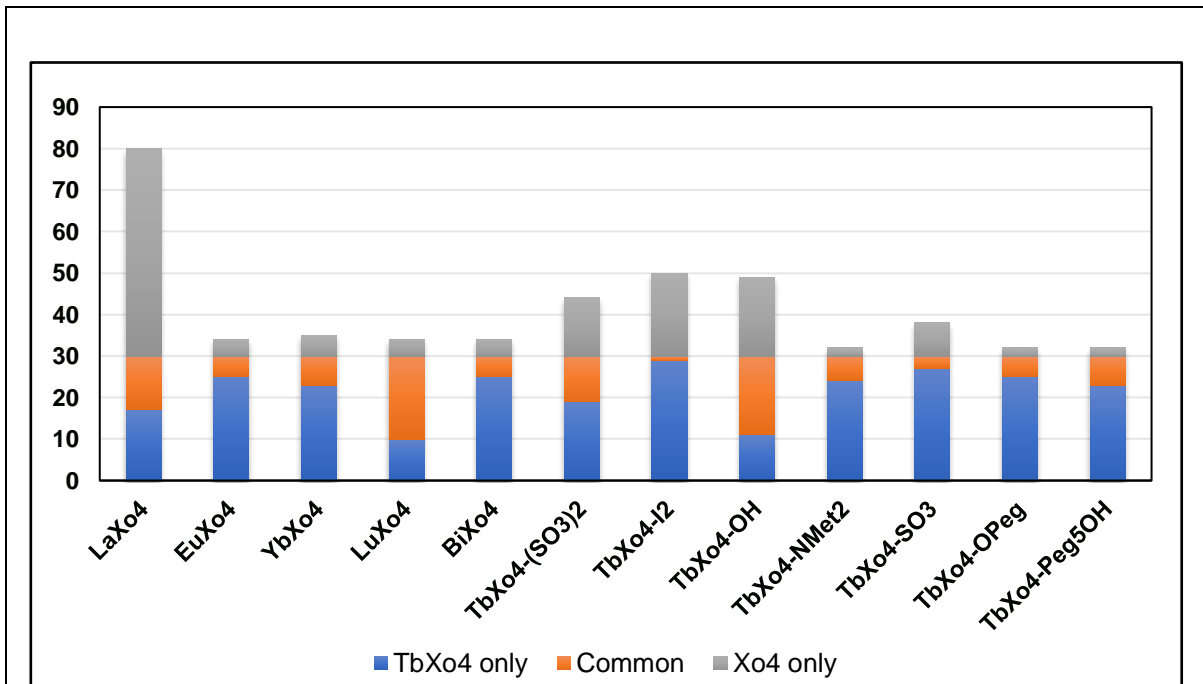
Figure 3-15 Comparison of variant versus TbXo4 crystallization outputs in the case of Thaumatin. Drop observation after 30 days: TbXo4 unique hits in blue, common hits (TbXo4 and Xo4 variants) in orange, Xo4 variants unique hits in grey.
