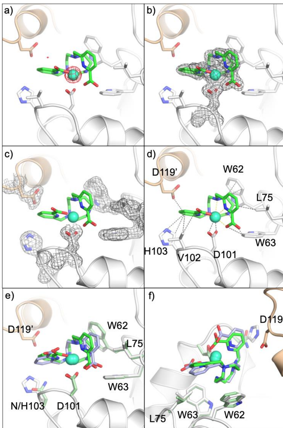
Figure 4-17 Structure of QEWL co-crystallized with 10 mM TbXo4. a) anomalous Fourier map (contour: 5 sigma) b) 2Fo-Fc electron density map superimposed to TbXo4 molecule (contour: 1 sigma) c) 2Fo-Fc electron density map corresponding to interaction sites of TbXo4 (1 sigma) d) Interaction sites of TbXo4. e-f) Superposition of TbXo4 in QEWL structure (TACN in green) and HEWL structure (palegreen) co-crystallized with 10 mM TbXo4 (TACN in lightblue). Tb atoms are represented as cyan sphere.
