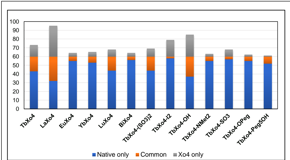
Figure 3-14 Results of the automated crystallization screening of crystallophore variants with Thaumatin after 30 days: number of unique hits for native protein in blue, common hits (native and Xo4) in orange, Xo4 variants unique hits in grey.
