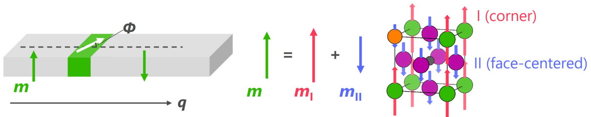
Figure 2.13: Image of the collective coordinate q - \phi model (1D model) expanded into a ferrimagnetic system with two sublattices, "I" and "II". In the case of \text{Mn}_{4-x}\text{Ni}_x\text{N} , we neglected the effect of magnetic moments of Ni, thus, the sublattice I and II consist of Mn(I) and Mn(II), respectively.
