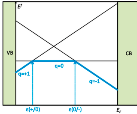
Figure 3.3: Schematic diagram presenting the variation of formation energy of a (hypothetical) defect with the value of electron chemical potential (Fermi energy) in charge state (q) +1, neutral, and -1. The thick blue solid lines represent the thermodynamically most stable charge state for a given Fermi energy. The charge transition levels (CTLs) within the band gap representing a change in the most stable charge state are marked with dashed lines. The Figure is reproduced from the the attached reference 40
