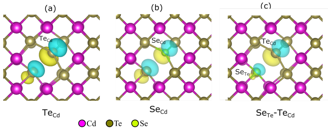
Figure 4.19: Kohn-Sham isosurfaces corresponding to (a) Te_{Cd} , (b) Se_{Cd} , and (c) Se_{Te}-Te_{Cd} antisite defects with electron density value of 0.005 \text{ e}/\text{\AA}^3 .
