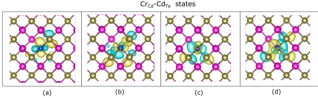
Figure 5.28: Kohn-Sham wavefunction isosurfaces corresponding to defect complex Cr_{Cd} - Cd_{Te} localised defect states lying close to band-edges with electron-density 0.0035 \text{ e}/\text{\AA}^3
