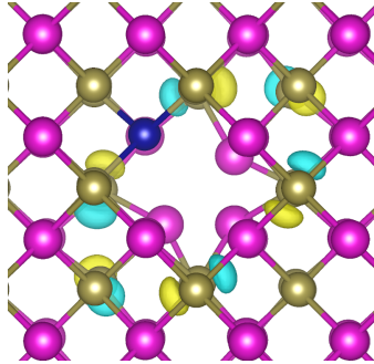
Figure 5.21: Kohn-Sham wavefunction isosurface of a_{1v} defect states of Cr_{Cd} - V_{Te} defect complex with electron-density of 0.002 e/\text{Å}^3
