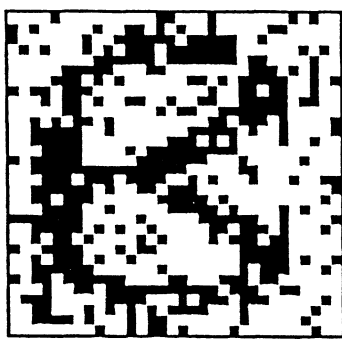
noisy image
