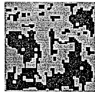
(c) \beta = 0.3(26\%)
